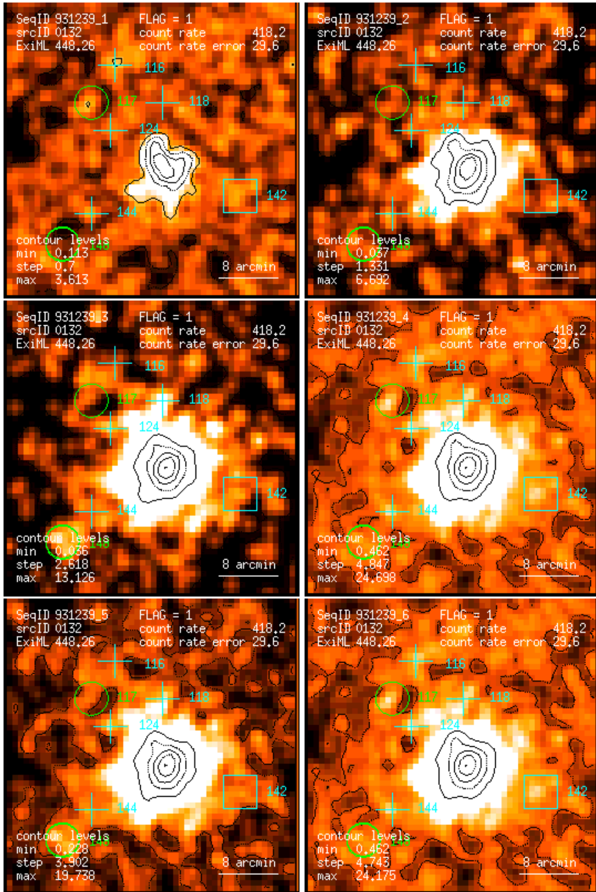
Figure 132: RASS 931239: detection 0132: band rate images, Gaussian filter: (1) PSPC channels 11 – 41, (2) 52 – 90, (3) 91 – 201, (4) 11 – 235, (5) 52 – 201, (6) 11 – 201. Broad band rates in counts/ks. Band rate contour levels in counts/ks/arcmin 2 .
