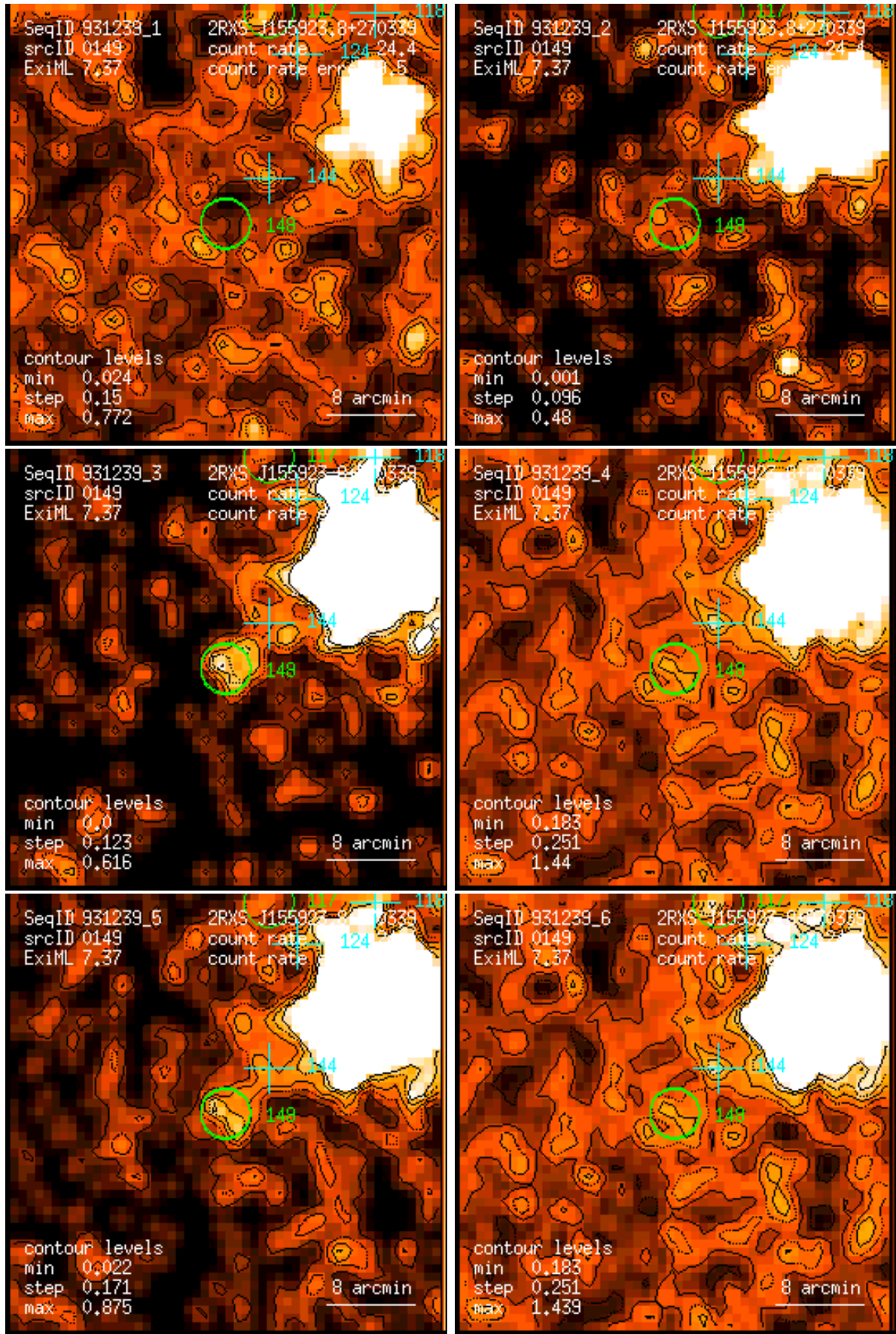
Figure 149: RASS 931239: detection 0149: band rate images, Gaussian filter: (1) PSPC channels 11 – 41, (2) 52 – 90, (3) 91 – 201, (4) 11 – 235, (5) 52 – 201, (6) 11 – 201. Broad band rates in counts/ks. Band rate contour levels in counts/ks/arcmin 2 .
