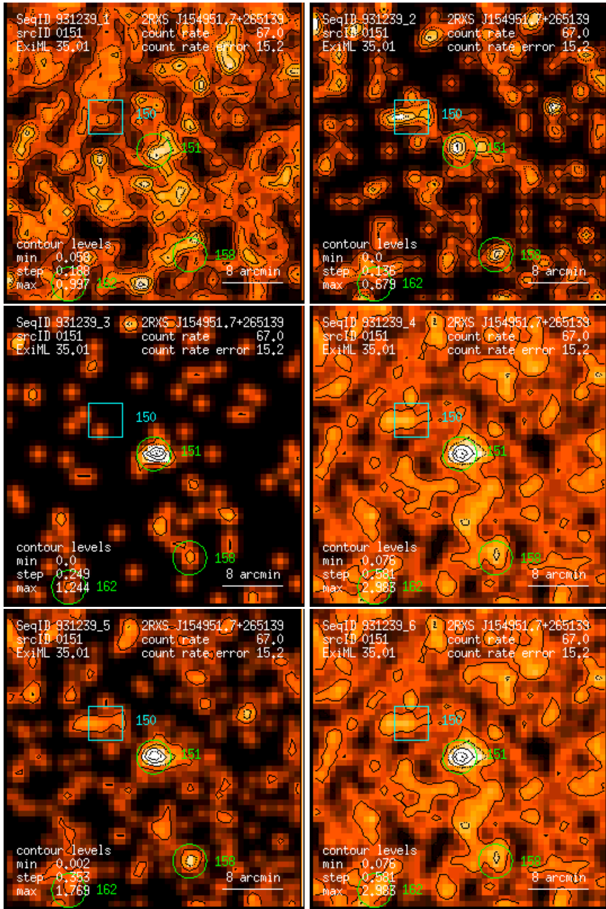
Figure 151: RASS 931239: detection 0151: band rate images, Gaussian filter: (1) PSPC channels 11 – 41, (2) 52 – 90, (3) 91 – 201, (4) 11 – 235, (5) 52 – 201, (6) 11 – 201. Broad band rates in counts/ks. Band rate contour levels in counts/ks/arcmin 2 .
