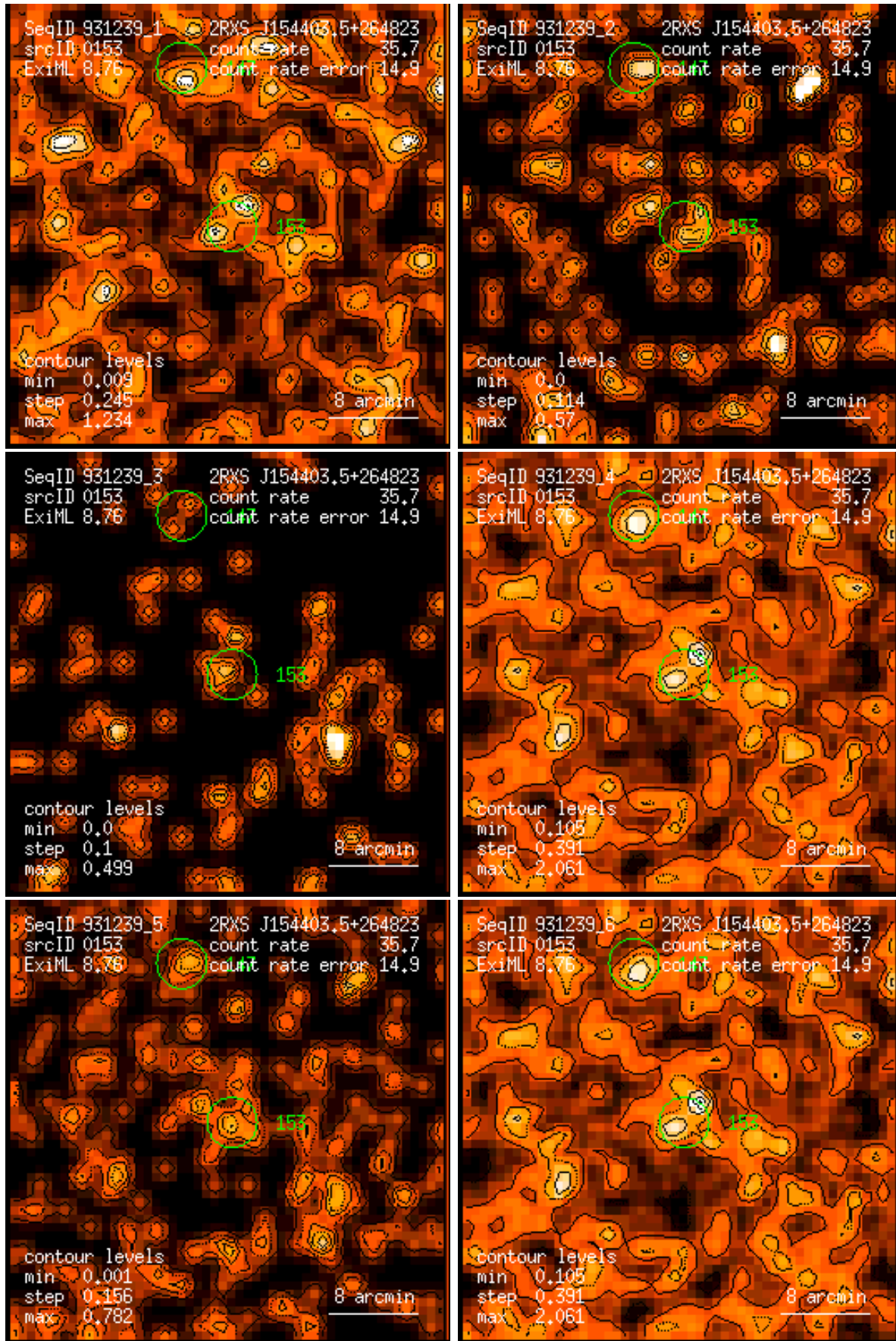
Figure 153: RASS 931239: detection 0153: band rate images, Gaussian filter: (1) PSPC channels 11 – 41, (2) 52 – 90, (3) 91 – 201, (4) 11 – 235, (5) 52 – 201, (6) 11 – 201. Broad band rates in counts/ks. Band rate contour levels in counts/ks/arcmin 2 .
