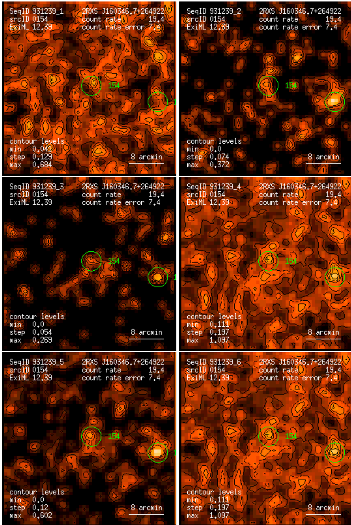
Figure 154: RASS 931239: detection 0154: band rate images, Gaussian filter: (1) PSPC channels 11 – 41, (2) 52 – 90, (3) 91 – 201, (4) 11 – 235, (5) 52 – 201, (6) 11 – 201. Broad band rates in counts/ks. Band rate contour levels in counts/ks/arcmin 2 .
