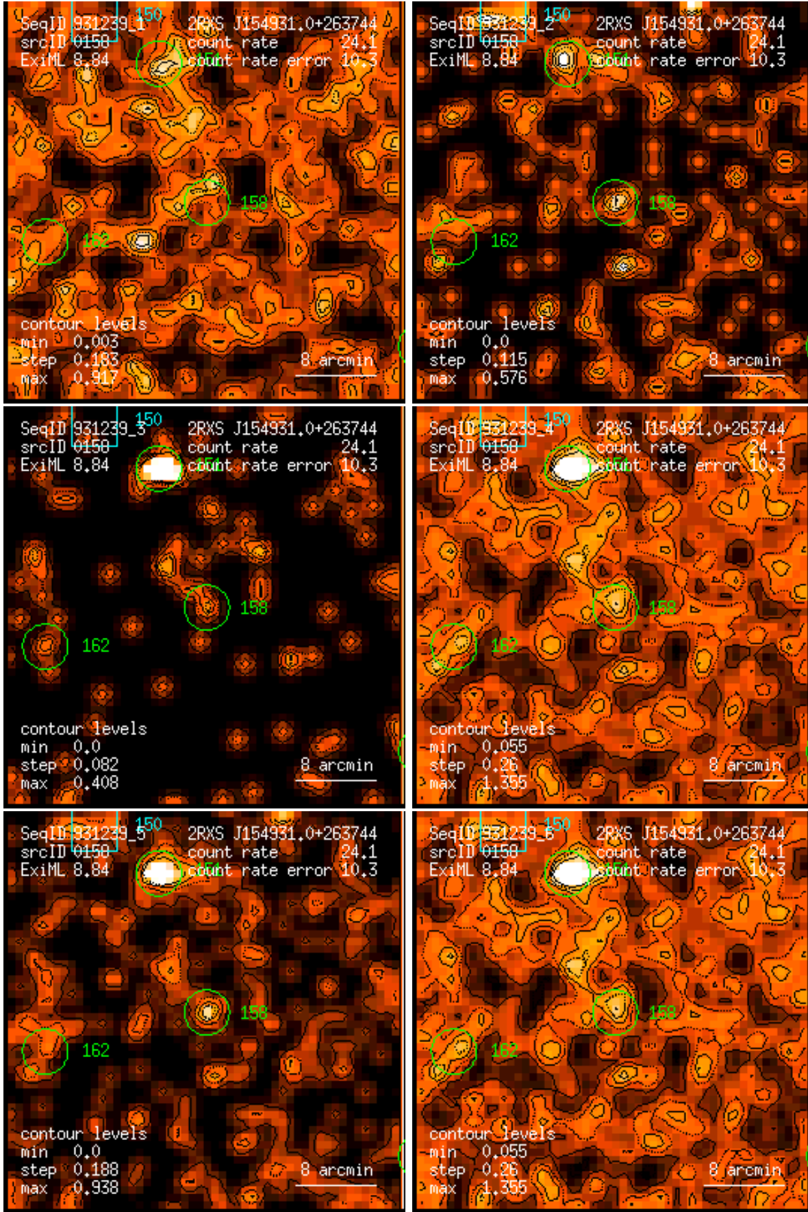
Figure 158: RASS 931239: detection 0158: band rate images, Gaussian filter: (1) PSPC channels 11 – 41, (2) 52 – 90, (3) 91 – 201, (4) 11 – 235, (5) 52 – 201, (6) 11 – 201. Broad band rates in counts/ks. Band rate contour levels in counts/ks/arcmin 2 .
