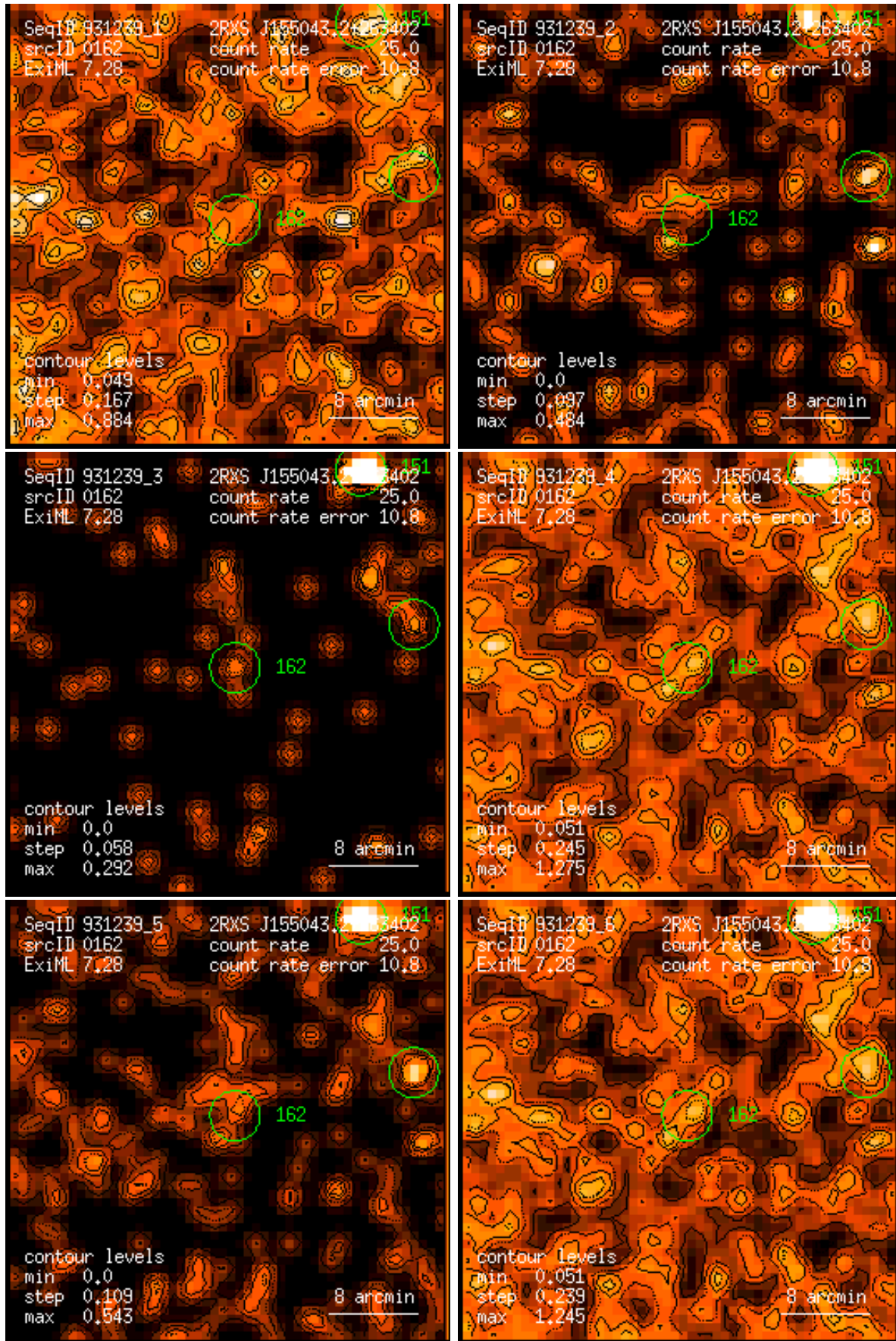
Figure 162: RASS 931239: detection 0162: band rate images, Gaussian filter: (1) PSPC channels 11 – 41, (2) 52 – 90, (3) 91 – 201, (4) 11 – 235, (5) 52 – 201, (6) 11 – 201. Broad band rates in counts/ks. Band rate contour levels in counts/ks/arcmin 2 .
