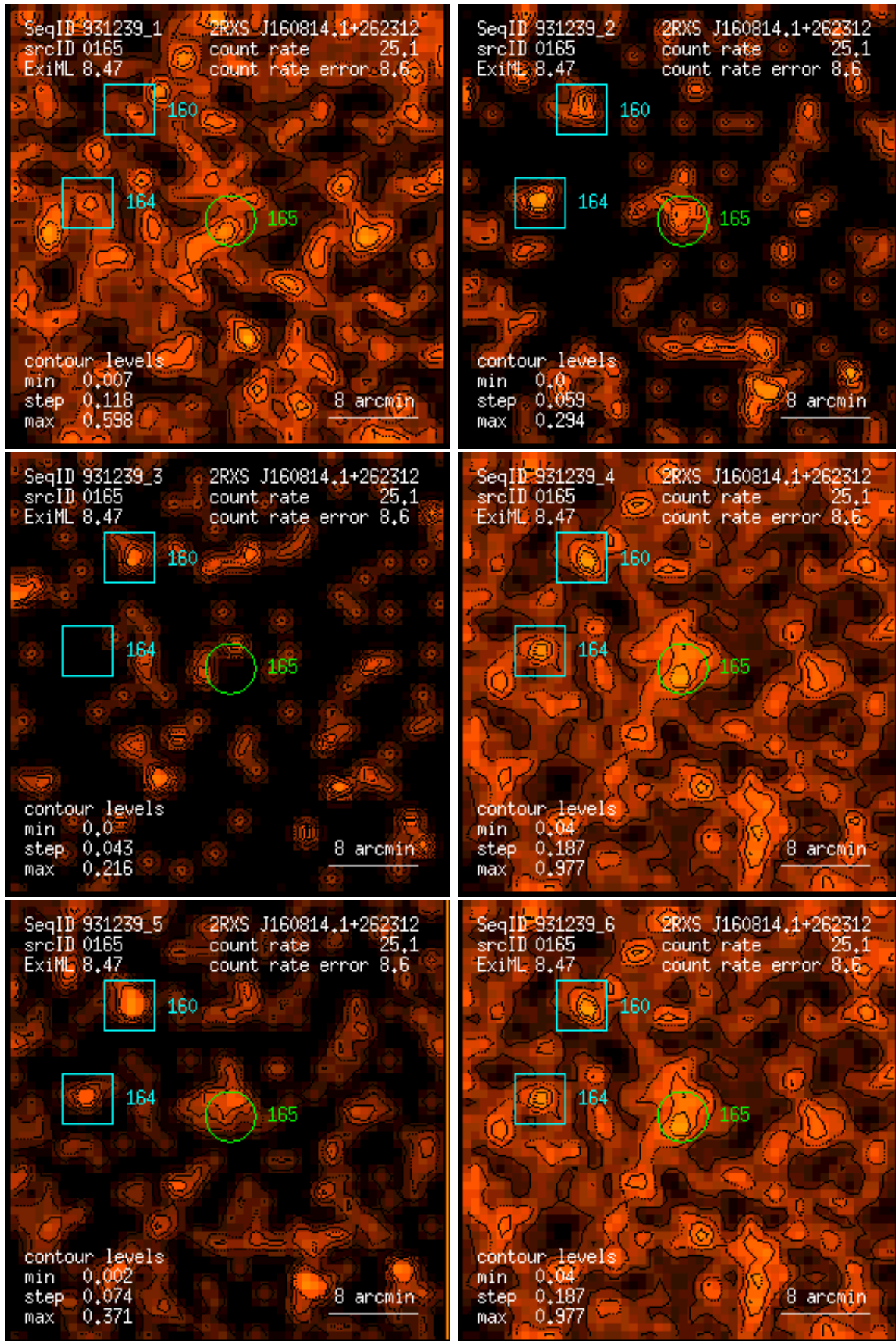
Figure 165: RASS 931239: detection 0165: band rate images, Gaussian filter: (1) PSPC channels 11 – 41, (2) 52 – 90, (3) 91 – 201, (4) 11 – 235, (5) 52 – 201, (6) 11 – 201. Broad band rates in counts/ks. Band rate contour levels in counts/ks/arcmin 2 .
