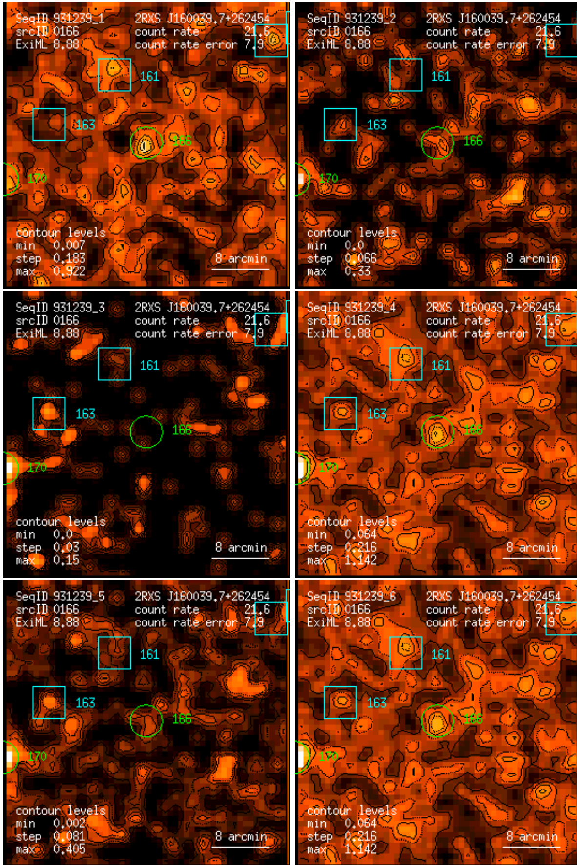
Figure 166: RASS 931239: detection 0166: band rate images, Gaussian filter: (1) PSPC channels 11 – 41, (2) 52 – 90, (3) 91 – 201, (4) 11 – 235, (5) 52 – 201, (6) 11 – 201. Broad band rates in counts/ks. Band rate contour levels in counts/ks/arcmin 2 .
