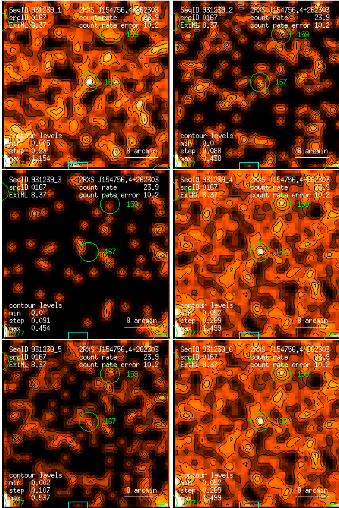
Figure 167: RASS 931239: detection 0167: band rate images, Gaussian filter: (1) PSPC channels 11 – 41, (2) 52 – 90, (3) 91 – 201, (4) 11 – 235, (5) 52 – 201, (6) 11 – 201. Broad band rates in counts/ks. Band rate contour levels in counts/ks/arcmin 2 .
