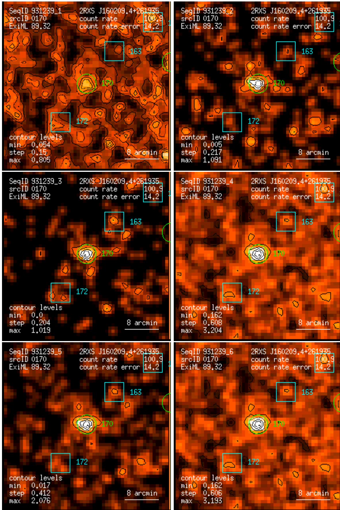
Figure 170: RASS 931239: detection 0170: band rate images, Gaussian filter: (1) PSPC channels 11 – 41, (2) 52 – 90, (3) 91 – 201, (4) 11 – 235, (5) 52 – 201, (6) 11 – 201. Broad band rates in counts/ks. Band rate contour levels in counts/ks/arcmin 2 .
