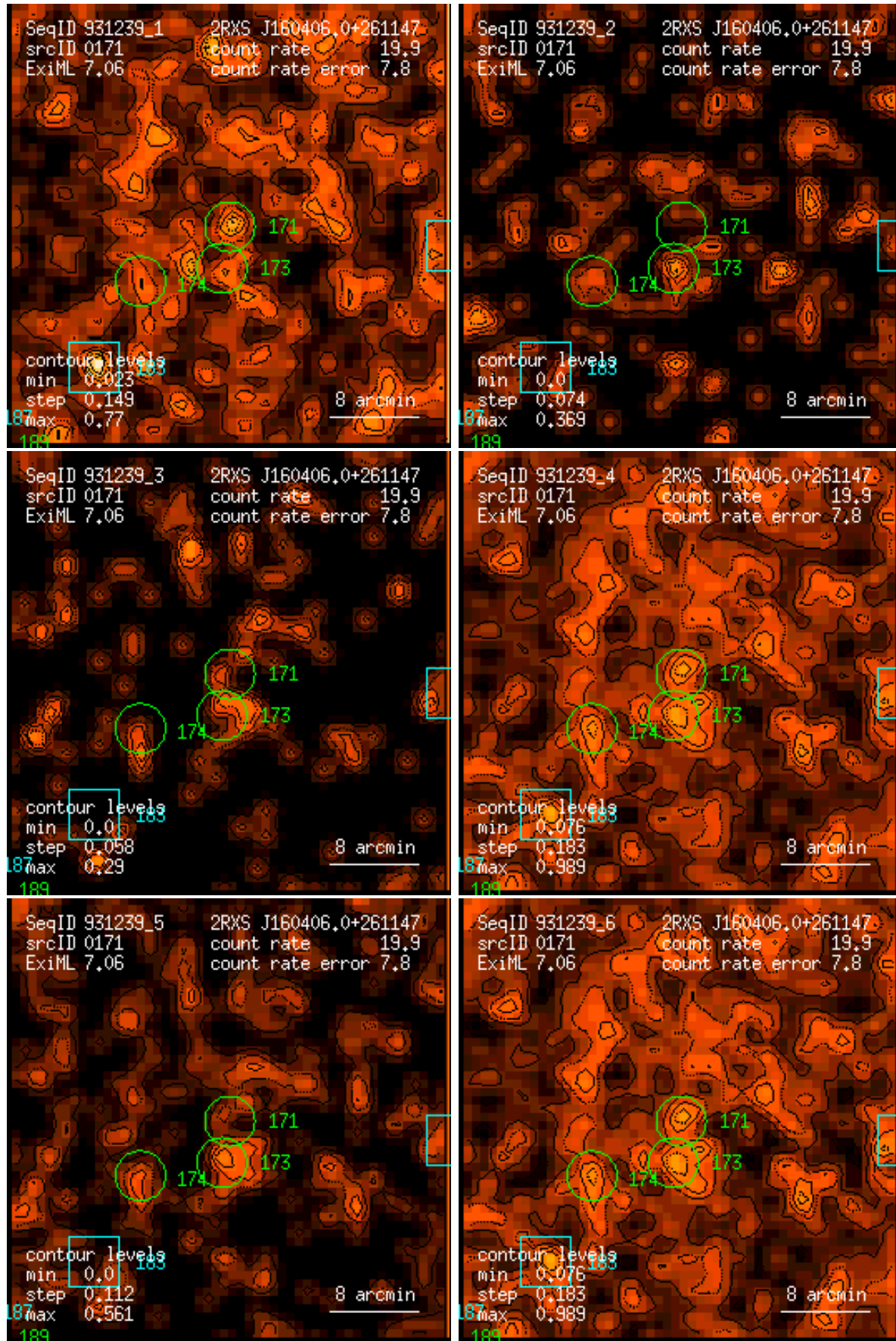
Figure 171: RASS 931239: detection 0171: band rate images, Gaussian filter: (1) PSPC channels 11 – 41, (2) 52 – 90, (3) 91 – 201, (4) 11 – 235, (5) 52 – 201, (6) 11 – 201. Broad band rates in counts/ks. Band rate contour levels in counts/ks/arcmin 2 .
