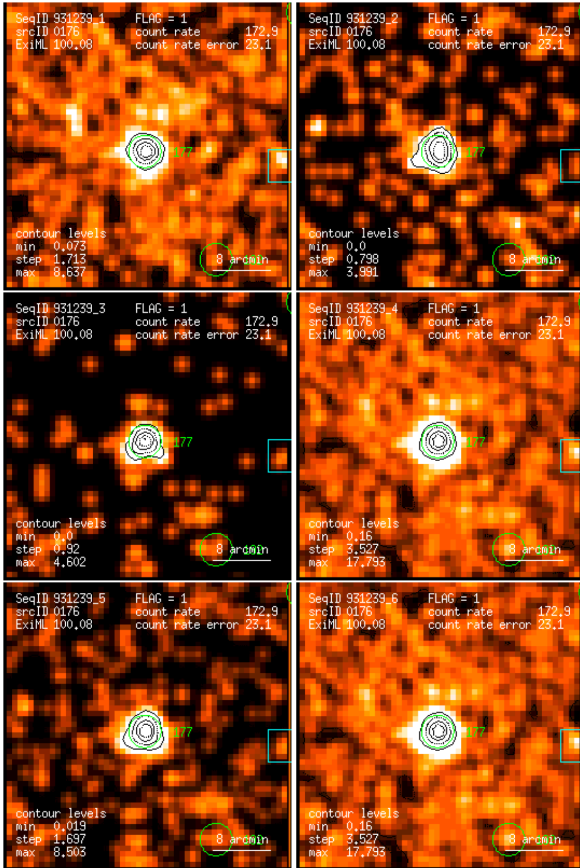
Figure 176: RASS 931239: detection 0176: band rate images, Gaussian filter: (1) PSPC channels 11 – 41, (2) 52 – 90, (3) 91 – 201, (4) 11 – 235, (5) 52 – 201, (6) 11 – 201. Broad band rates in counts/ks. Band rate contour levels in counts/ks/arcmin 2 .
