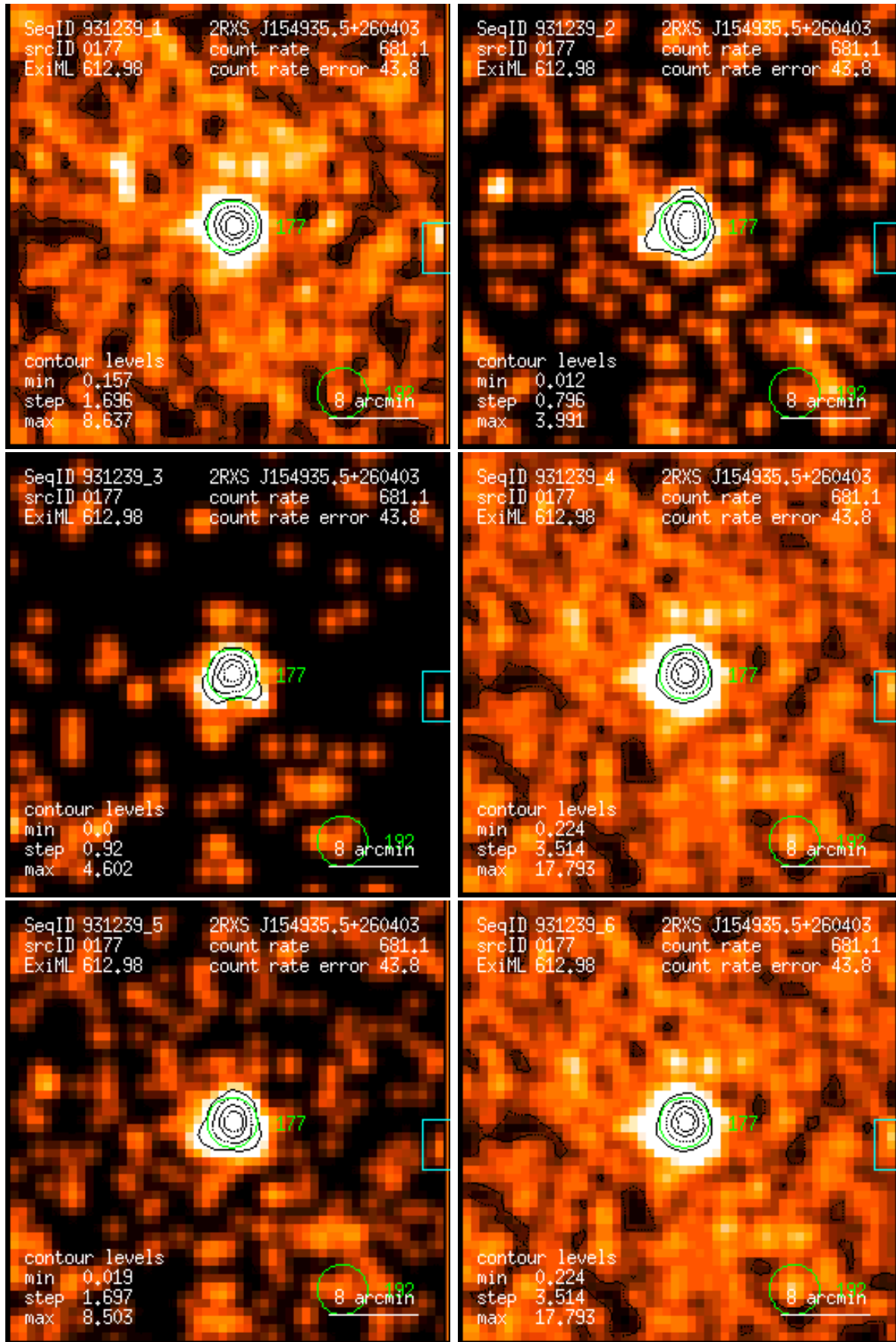
Figure 177: RASS 931239: detection 0177: band rate images, Gaussian filter: (1) PSPC channels 11 – 41, (2) 52 – 90, (3) 91 – 201, (4) 11 – 235, (5) 52 – 201, (6) 11 – 201. Broad band rates in counts/ks. Band rate contour levels in counts/ks/arcmin 2 .
