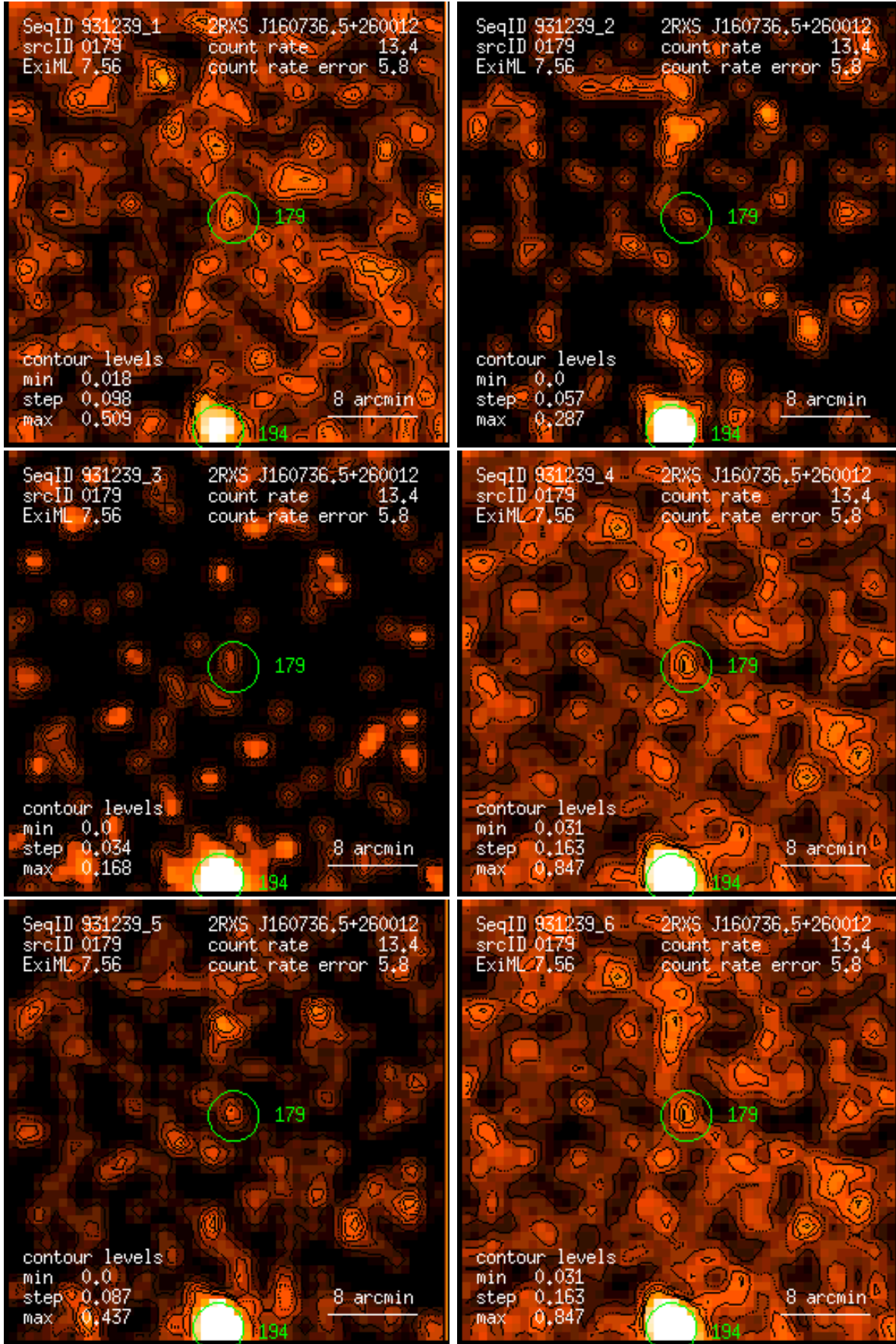
Figure 179: RASS 931239: detection 0179: band rate images, Gaussian filter: (1) PSPC channels 11 – 41, (2) 52 – 90, (3) 91 – 201, (4) 11 – 235, (5) 52 – 201, (6) 11 – 201. Broad band rates in counts/ks. Band rate contour levels in counts/ks/arcmin 2 .
