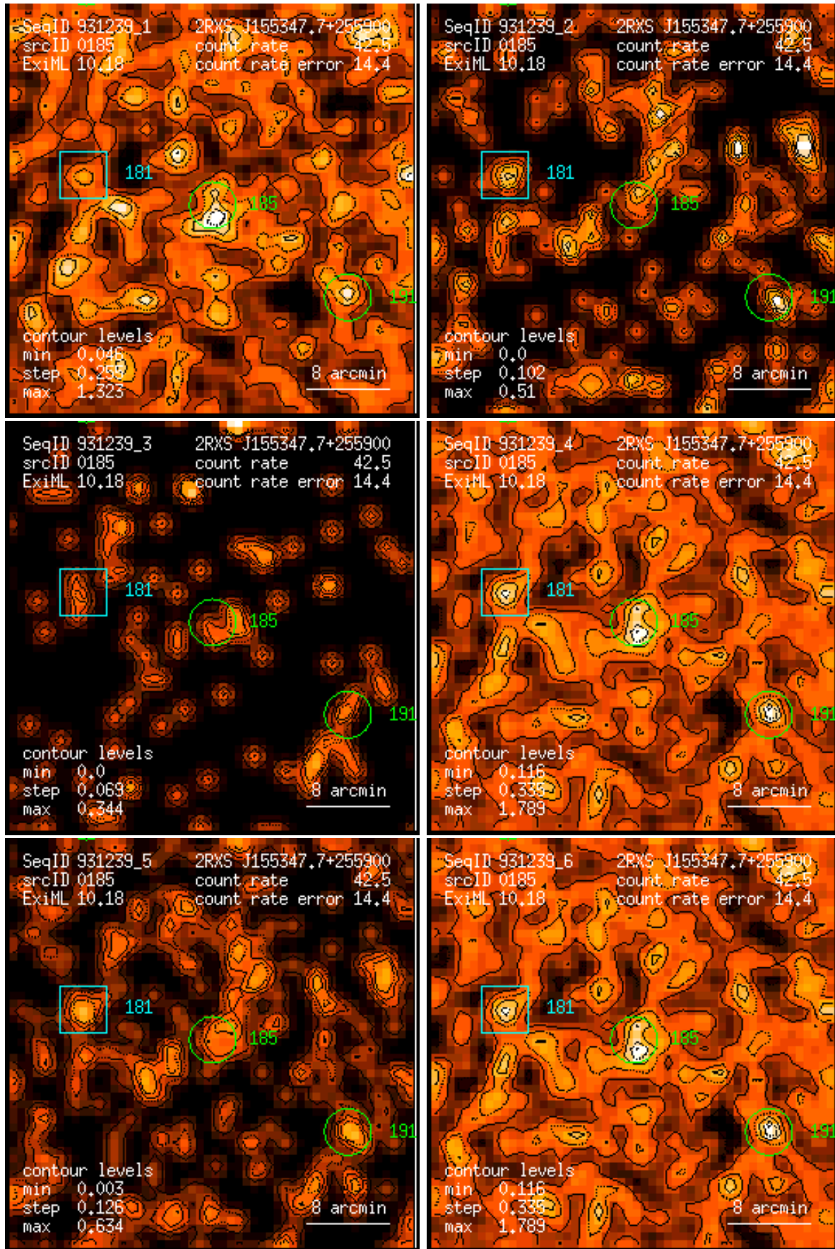
Figure 185: RASS 931239: detection 0185: band rate images, Gaussian filter: (1) PSPC channels 11 – 41, (2) 52 – 90, (3) 91 – 201, (4) 11 – 235, (5) 52 – 201, (6) 11 – 201. Broad band rates in counts/ks. Band rate contour levels in counts/ks/arcmin 2 .
