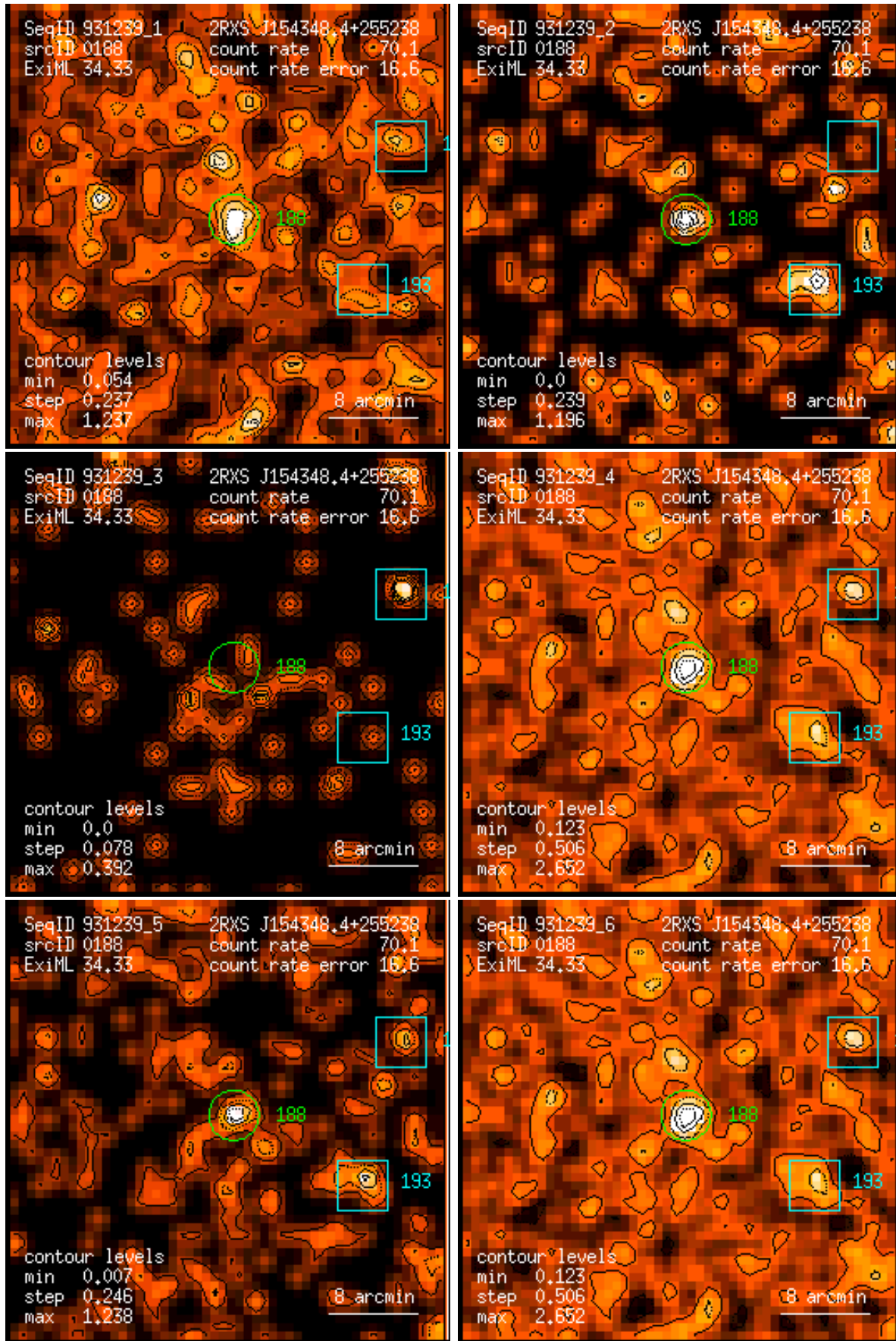
Figure 188: RASS 931239: detection 0188: band rate images, Gaussian filter: (1) PSPC channels 11 – 41, (2) 52 – 90, (3) 91 – 201, (4) 11 – 235, (5) 52 – 201, (6) 11 – 201. Broad band rates in counts/ks. Band rate contour levels in counts/ks/arcmin 2 .
