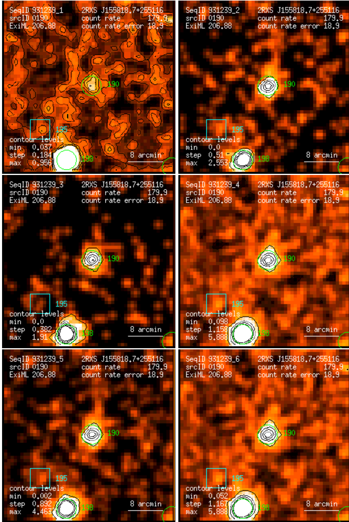
Figure 190: RASS 931239: detection 0190: band rate images, Gaussian filter: (1) PSPC channels 11 – 41, (2) 52 – 90, (3) 91 – 201, (4) 11 – 235, (5) 52 – 201, (6) 11 – 201. Broad band rates in counts/ks. Band rate contour levels in counts/ks/arcmin 2 .
