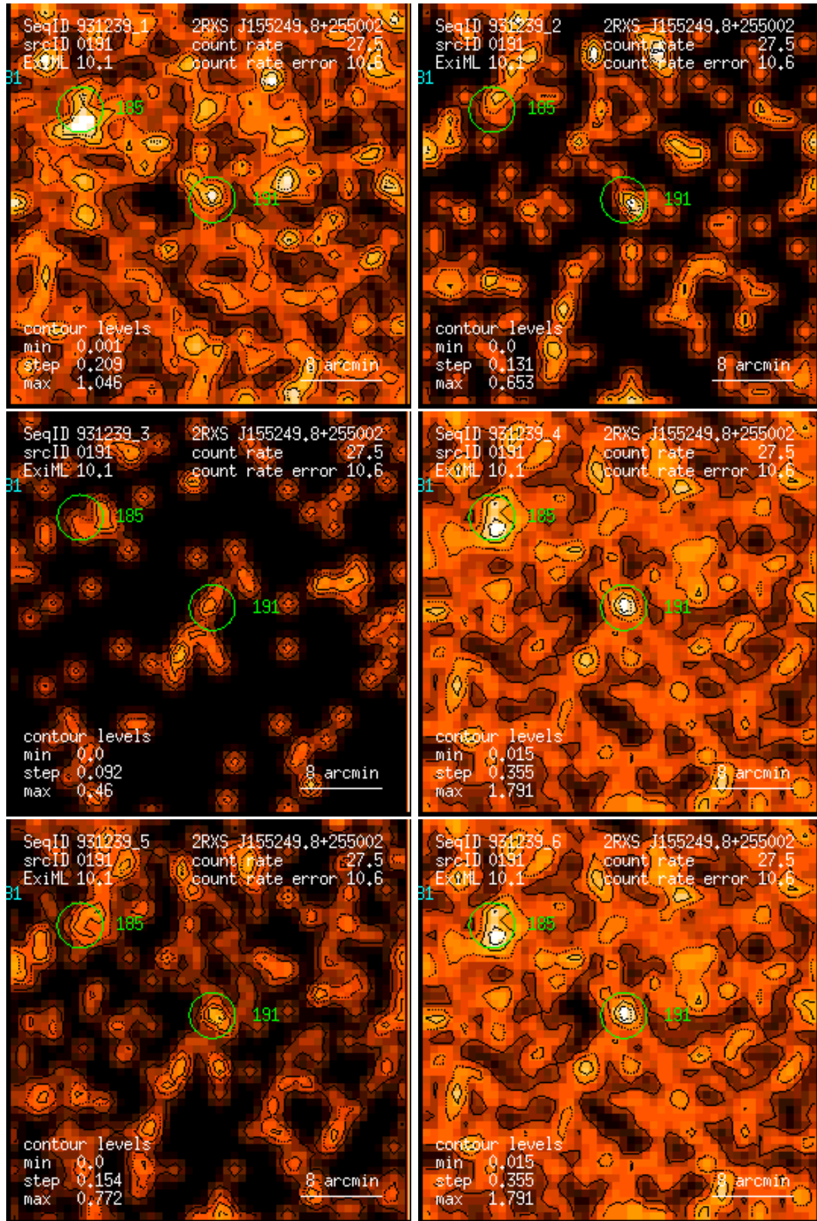
Figure 191: RASS 931239: detection 0191: band rate images, Gaussian filter: (1) PSPC channels 11 – 41, (2) 52 – 90, (3) 91 – 201, (4) 11 – 235, (5) 52 – 201, (6) 11 – 201. Broad band rates in counts/ks. Band rate contour levels in counts/ks/arcmin 2 .
