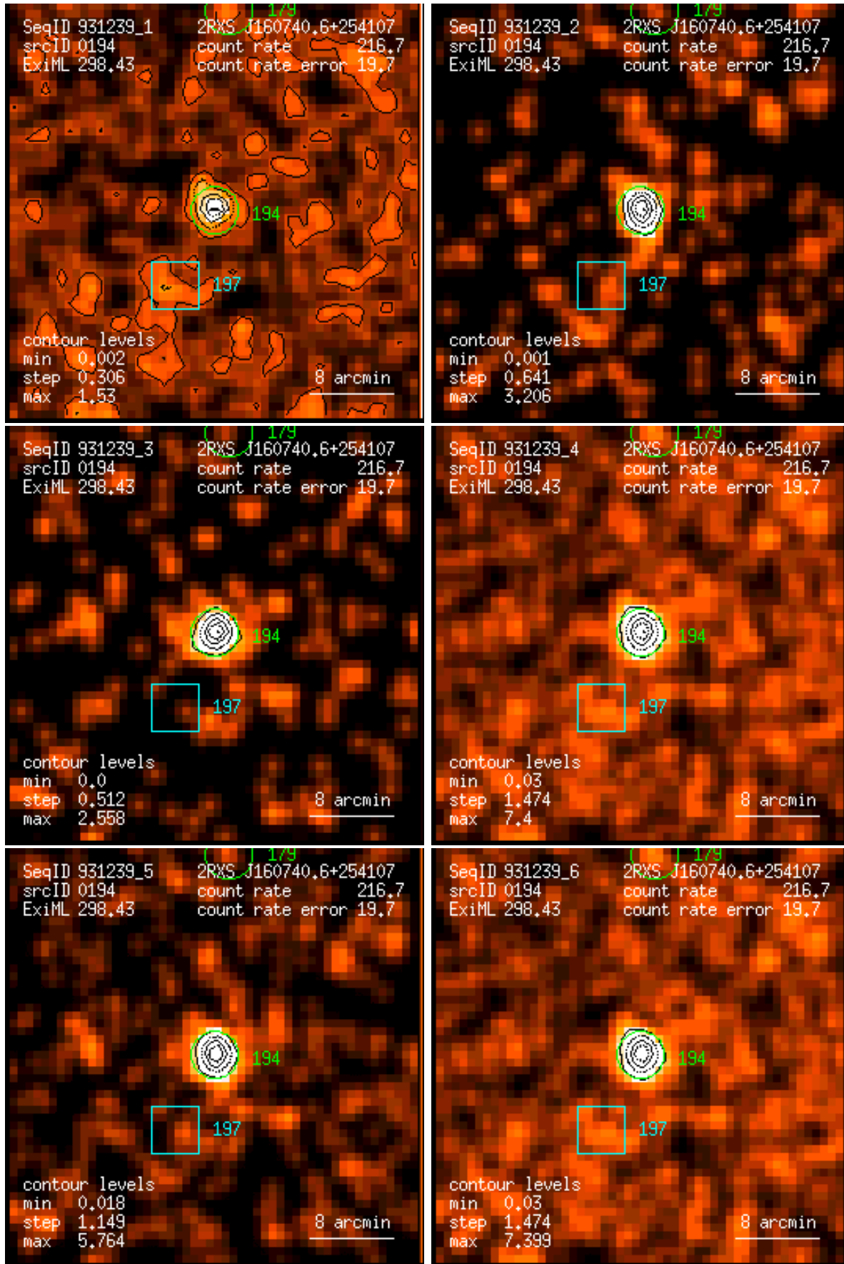
Figure 194: RASS 931239: detection 0194: band rate images, Gaussian filter: (1) PSPC channels 11 – 41, (2) 52 – 90, (3) 91 – 201, (4) 11 – 235, (5) 52 – 201, (6) 11 – 201. Broad band rates in counts/ks. Band rate contour levels in counts/ks/arcmin 2 .
