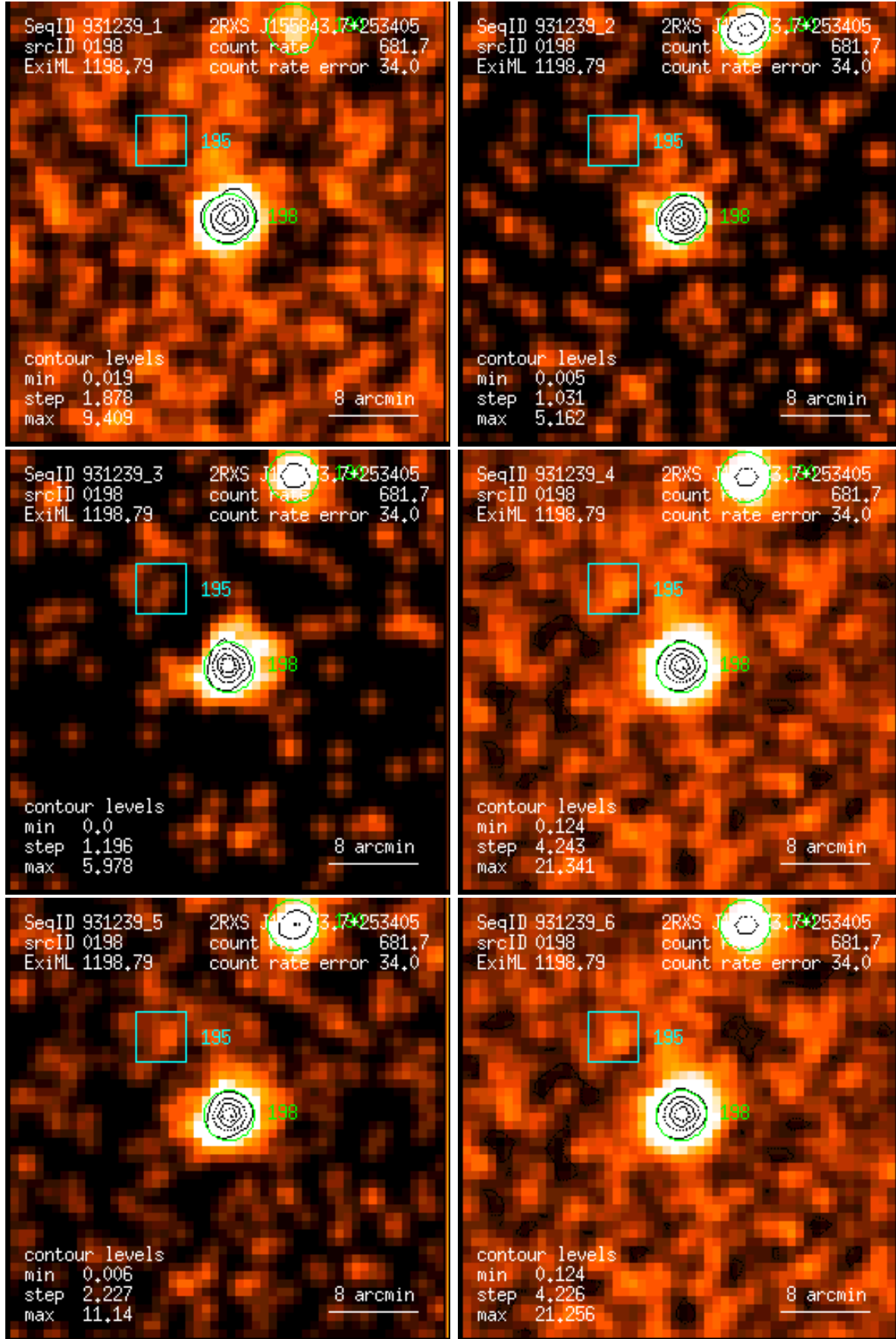
Figure 198: RASS 931239: detection 0198: band rate images, Gaussian filter: (1) PSPC channels 11 – 41, (2) 52 – 90, (3) 91 – 201, (4) 11 – 235, (5) 52 – 201, (6) 11 – 201. Broad band rates in counts/ks. Band rate contour levels in counts/ks/arcmin 2 .
