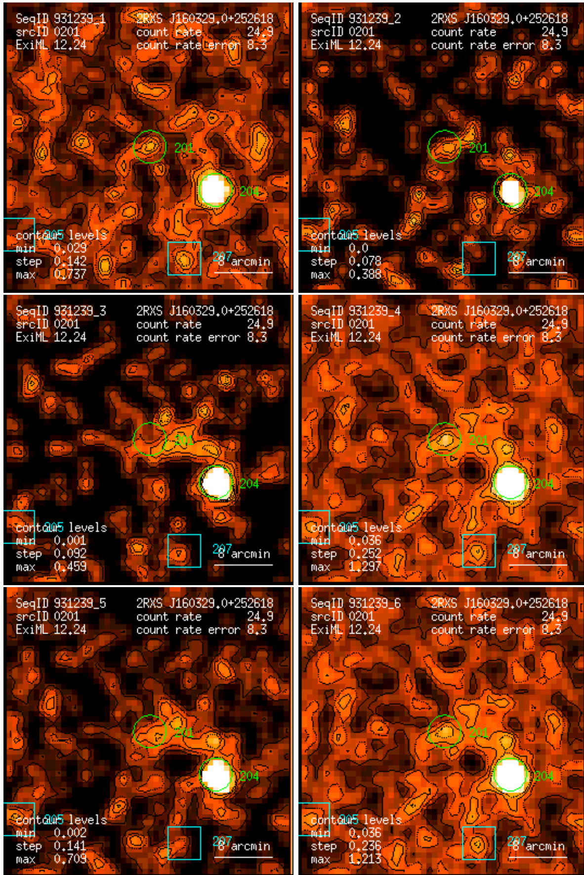
Figure 201: RASS 931239: detection 0201: band rate images, Gaussian filter: (1) PSPC channels 11 – 41, (2) 52 – 90, (3) 91 – 201, (4) 11 – 235, (5) 52 – 201, (6) 11 – 201. Broad band rates in counts/ks. Band rate contour levels in counts/ks/arcmin 2 .
