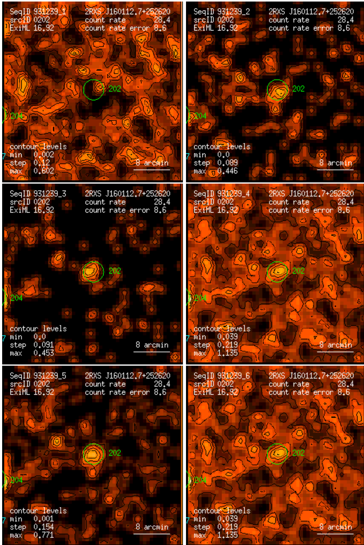
Figure 202: RASS 931239: detection 0202: band rate images, Gaussian filter: (1) PSPC channels 11 – 41, (2) 52 – 90, (3) 91 – 201, (4) 11 – 235, (5) 52 – 201, (6) 11 – 201. Broad band rates in counts/ks. Band rate contour levels in counts/ks/arcmin 2 .
