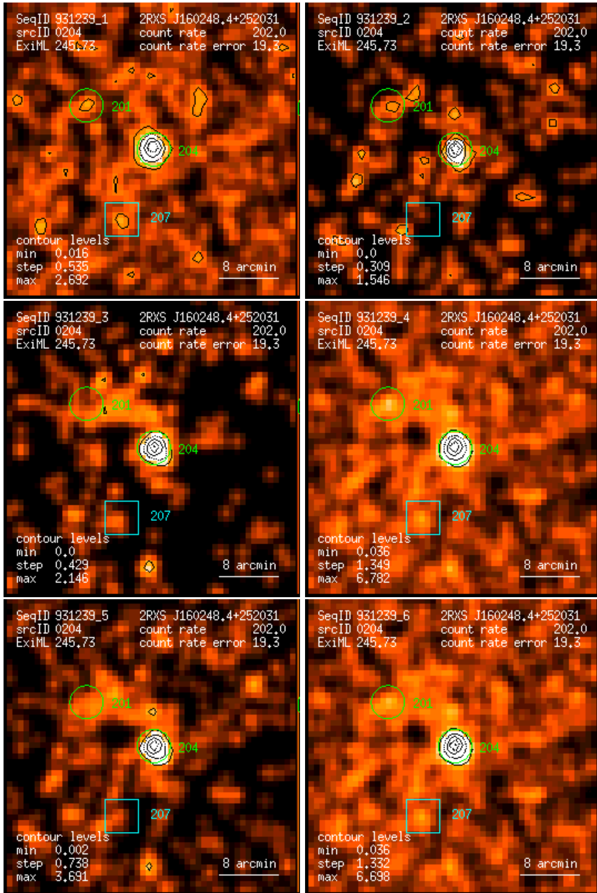
Figure 204: RASS 931239: detection 0204: band rate images, Gaussian filter: (1) PSPC channels 11 – 41, (2) 52 – 90, (3) 91 – 201, (4) 11 – 235, (5) 52 – 201, (6) 11 – 201. Broad band rates in counts/ks. Band rate contour levels in counts/ks/arcmin 2 .
