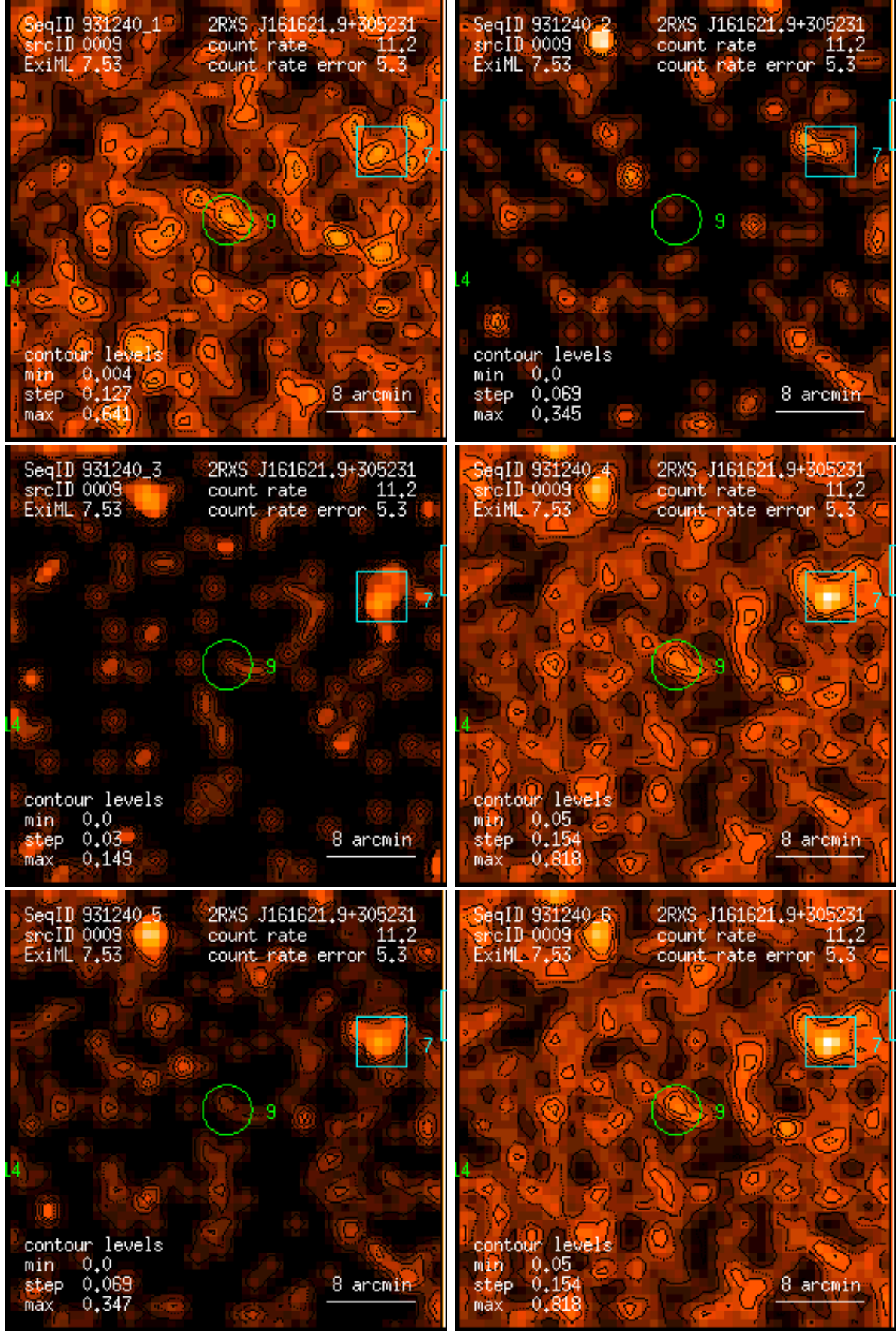
Figure 9: RASS 931240: detection 0009: band rate images, Gaussian filter: (1) PSPC channels 11 – 41, (2) 52 – 90, (3) 91 – 201, (4) 11 – 235, (5) 52 – 201, (6) 11 – 201. Broad band rates in counts/ks. Band rate contour levels in counts/ks/arcmin 2 .
