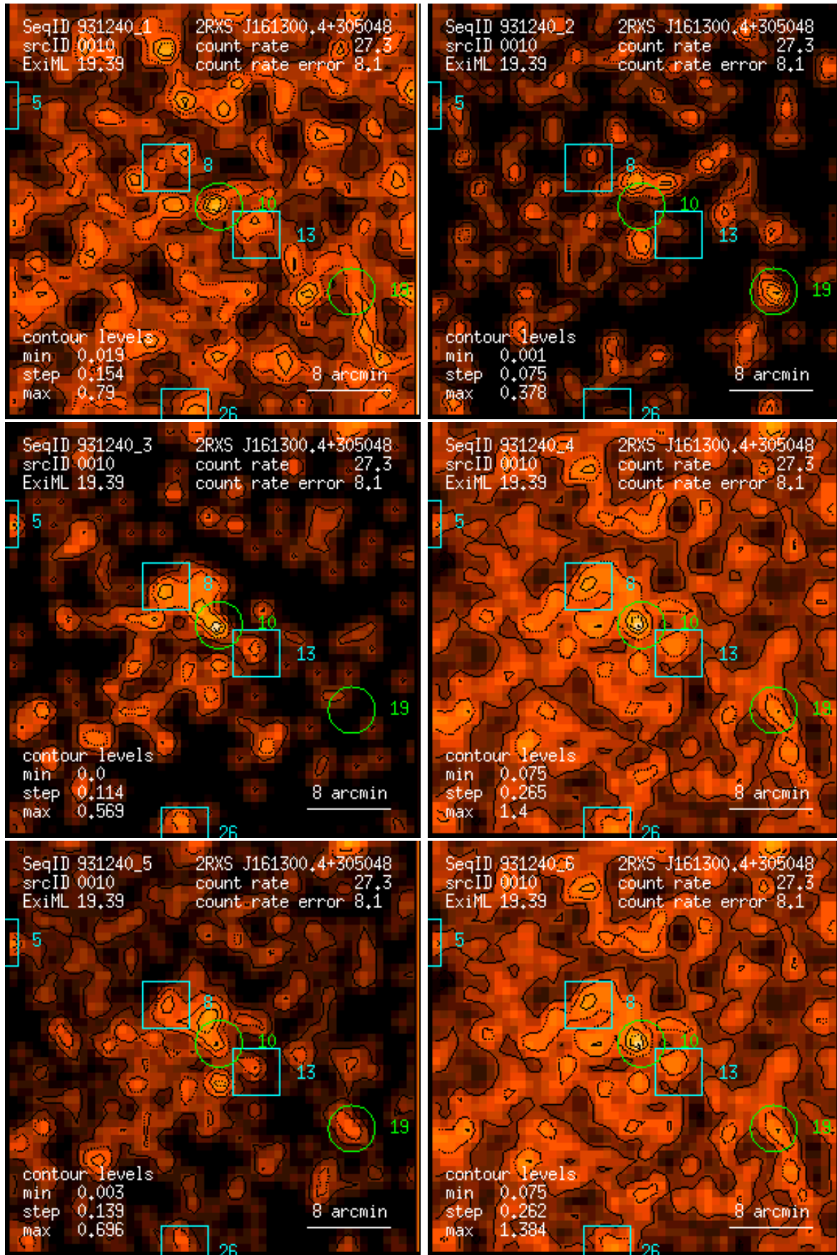
Figure 10: RASS 931240: detection 0010: band rate images, Gaussian filter: (1) PSPC channels 11 – 41, (2) 52 – 90, (3) 91 – 201, (4) 11 – 235, (5) 52 – 201, (6) 11 – 201. Broad band rates in counts/ks. Band rate contour levels in counts/ks/arcmin 2 .
