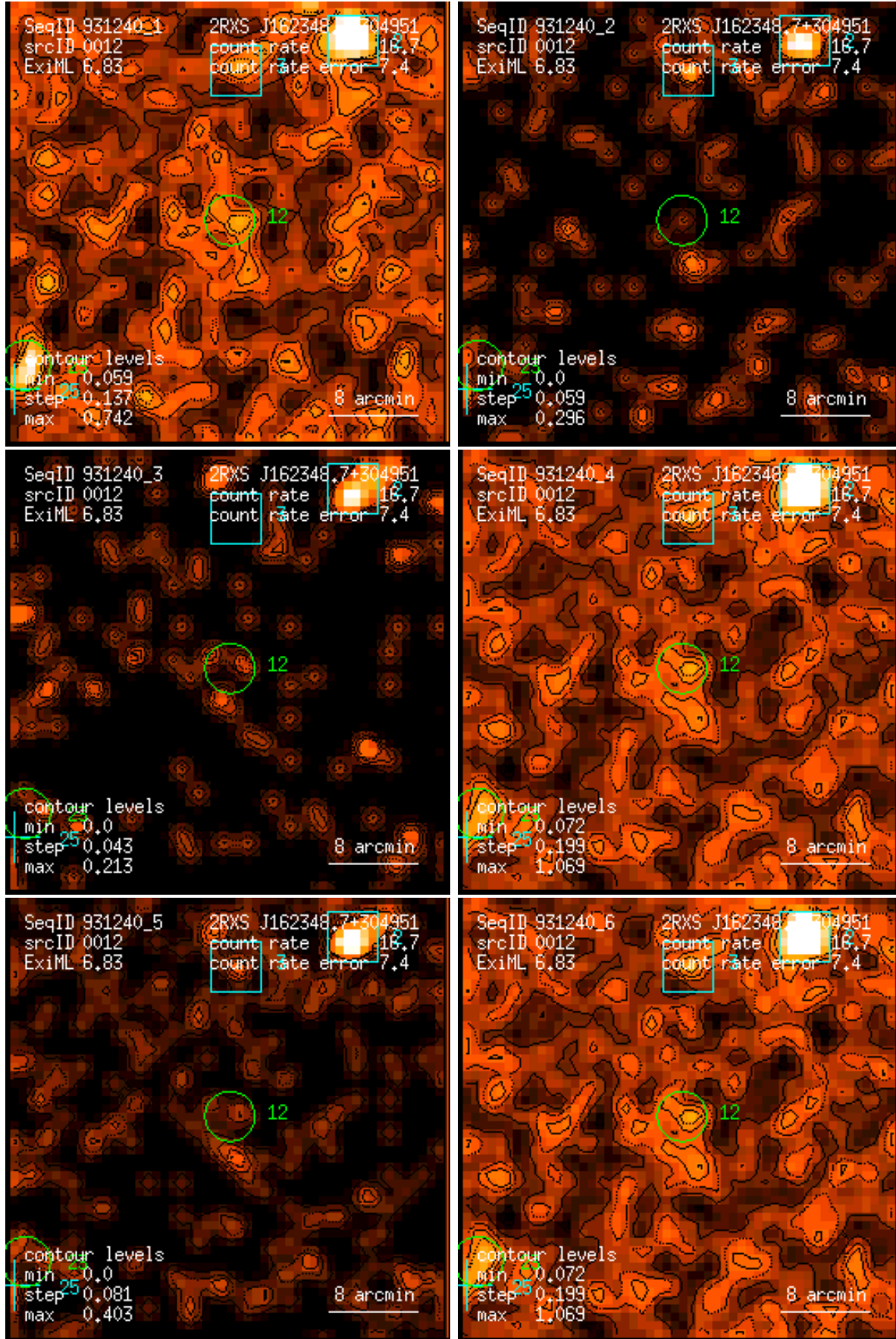
Figure 12: RASS 931240: detection 0012: band rate images, Gaussian filter: (1) PSPC channels 11 – 41, (2) 52 – 90, (3) 91 – 201, (4) 11 – 235, (5) 52 – 201, (6) 11 – 201. Broad band rates in counts/ks. Band rate contour levels in counts/ks/arcmin 2 .
