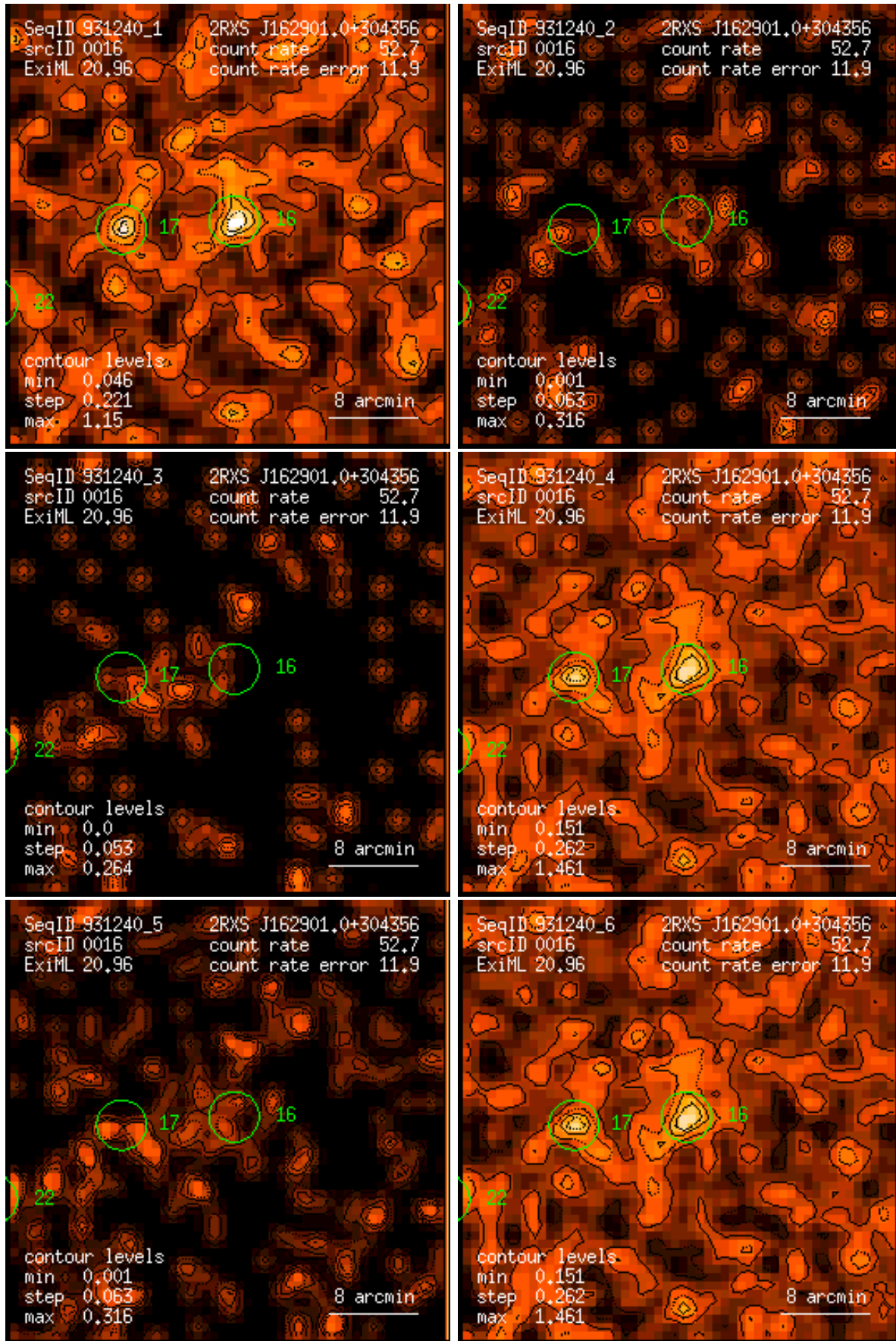
Figure 16: RASS 931240: detection 0016: band rate images, Gaussian filter: (1) PSPC channels 11 – 41, (2) 52 – 90, (3) 91 – 201, (4) 11 – 235, (5) 52 – 201, (6) 11 – 201. Broad band rates in counts/ks. Band rate contour levels in counts/ks/arcmin 2 .
