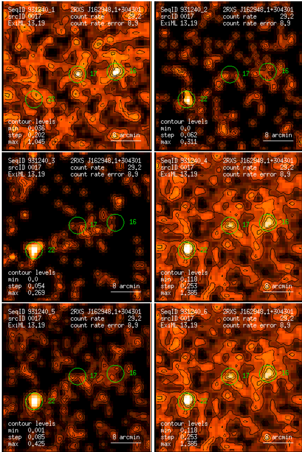
Figure 17: RASS 931240: detection 0017: band rate images, Gaussian filter: (1) PSPC channels 11 – 41, (2) 52 – 90, (3) 91 – 201, (4) 11 – 235, (5) 52 – 201, (6) 11 – 201. Broad band rates in counts/ks. Band rate contour levels in counts/ks/arcmin 2 .
