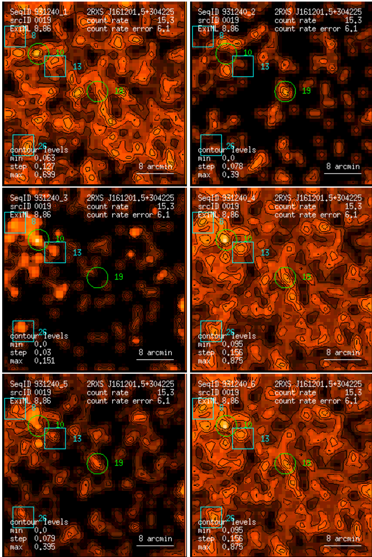
Figure 19: RASS 931240: detection 0019: band rate images, Gaussian filter: (1) PSPC channels 11 – 41, (2) 52 – 90, (3) 91 – 201, (4) 11 – 235, (5) 52 – 201, (6) 11 – 201. Broad band rates in counts/ks. Band rate contour levels in counts/ks/arcmin 2 .
