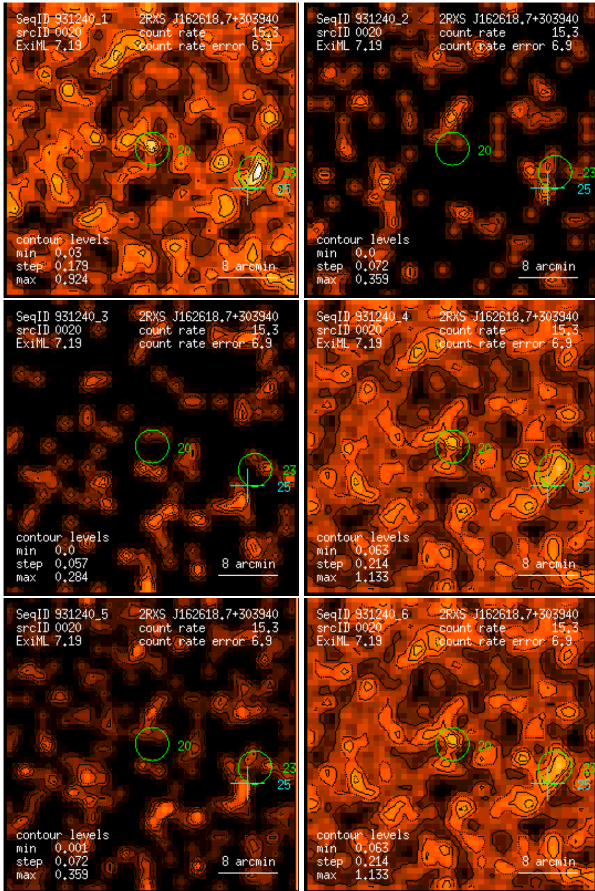
Figure 20: RASS 931240: detection 0020: band rate images, Gaussian filter: (1) PSPC channels 11 – 41, (2) 52 – 90, (3) 91 – 201, (4) 11 – 235, (5) 52 – 201, (6) 11 – 201. Broad band rates in counts/ks. Band rate contour levels in counts/ks/arcmin 2 .
