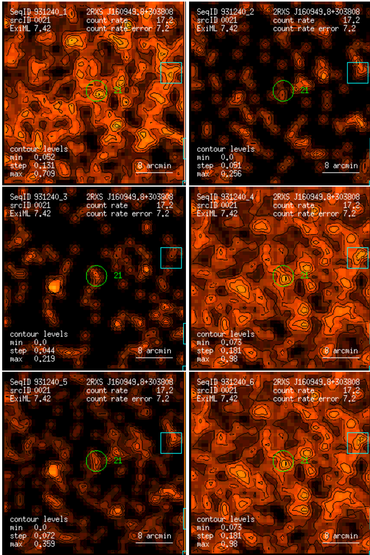
Figure 21: RASS 931240: detection 0021: band rate images, Gaussian filter: (1) PSPC channels 11 – 41, (2) 52 – 90, (3) 91 – 201, (4) 11 – 235, (5) 52 – 201, (6) 11 – 201. Broad band rates in counts/ks. Band rate contour levels in counts/ks/arcmin 2 .
