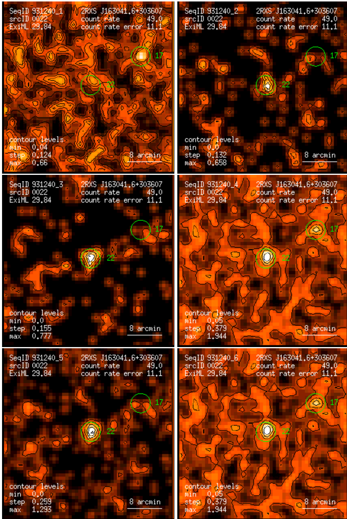
Figure 22: RASS 931240: detection 0022: band rate images, Gaussian filter: (1) PSPC channels 11 – 41, (2) 52 – 90, (3) 91 – 201, (4) 11 – 235, (5) 52 – 201, (6) 11 – 201. Broad band rates in counts/ks. Band rate contour levels in counts/ks/arcmin 2 .
