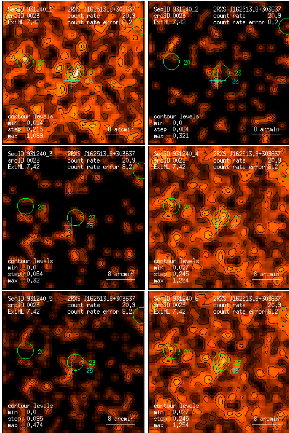
Figure 23: RASS 931240: detection 0023: band rate images, Gaussian filter: (1) PSPC channels 11 – 41, (2) 52 – 90, (3) 91 – 201, (4) 11 – 235, (5) 52 – 201, (6) 11 – 201. Broad band rates in counts/ks. Band rate contour levels in counts/ks/arcmin 2 .
