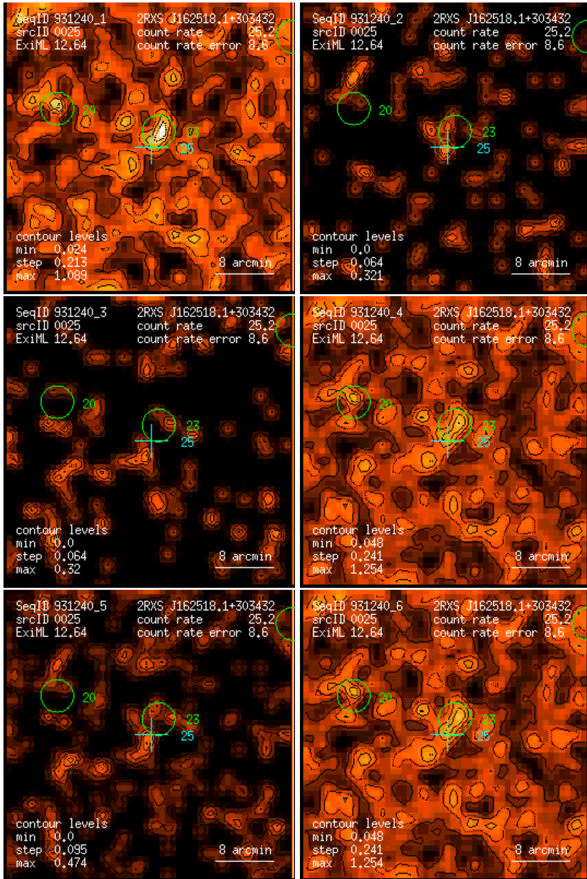
Figure 25: RASS 931240: detection 0025: band rate images, Gaussian filter: (1) PSPC channels 11 – 41, (2) 52 – 90, (3) 91 – 201, (4) 11 – 235, (5) 52 – 201, (6) 11 – 201. Broad band rates in counts/ks. Band rate contour levels in counts/ks/arcmin 2 .
