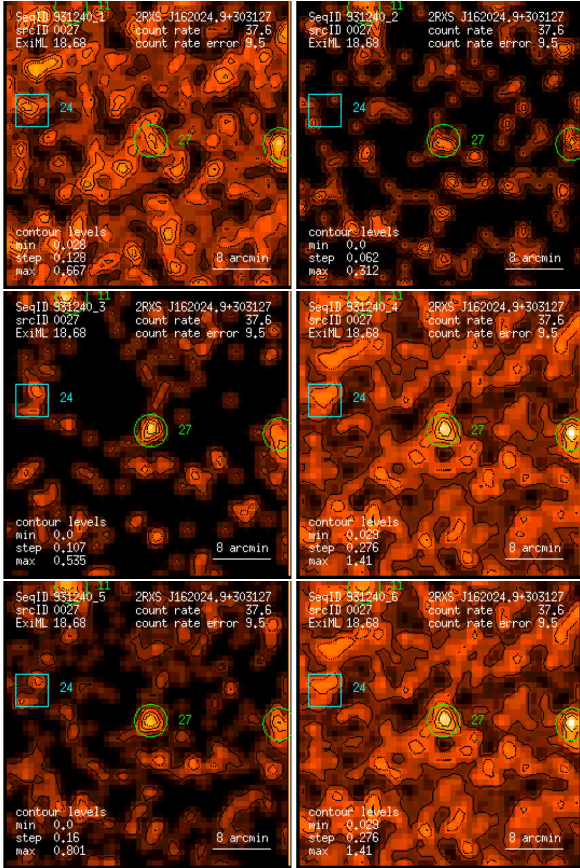
Figure 27: RASS 931240: detection 0027: band rate images, Gaussian filter: (1) PSPC channels 11 – 41, (2) 52 – 90, (3) 91 – 201, (4) 11 – 235, (5) 52 – 201, (6) 11 – 201. Broad band rates in counts/ks. Band rate contour levels in counts/ks/arcmin 2 .
