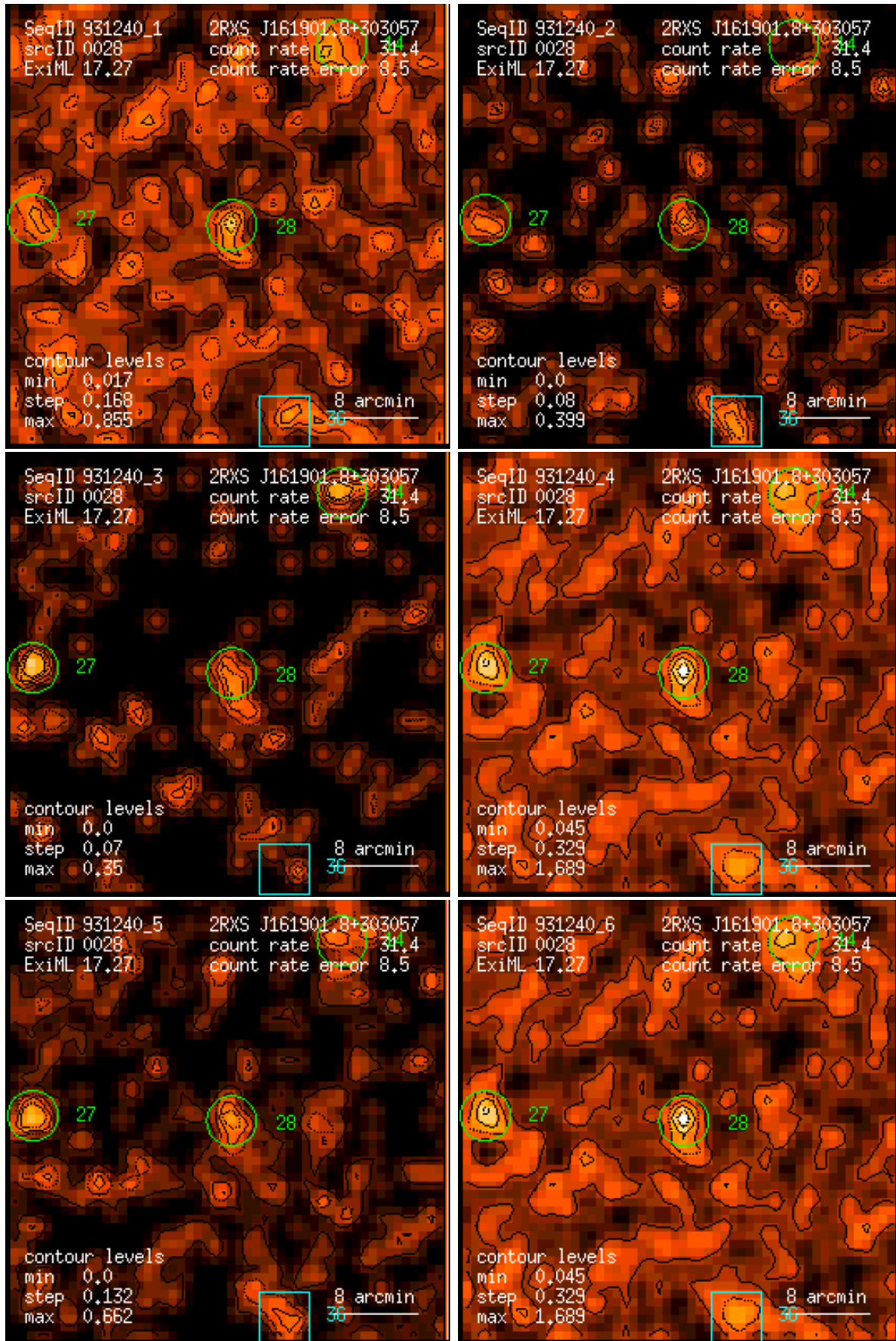
Figure 28: RASS 931240: detection 0028: band rate images, Gaussian filter: (1) PSPC channels 11 – 41, (2) 52 – 90, (3) 91 – 201, (4) 11 – 235, (5) 52 – 201, (6) 11 – 201. Broad band rates in counts/ks. Band rate contour levels in counts/ks/arcmin 2 .
