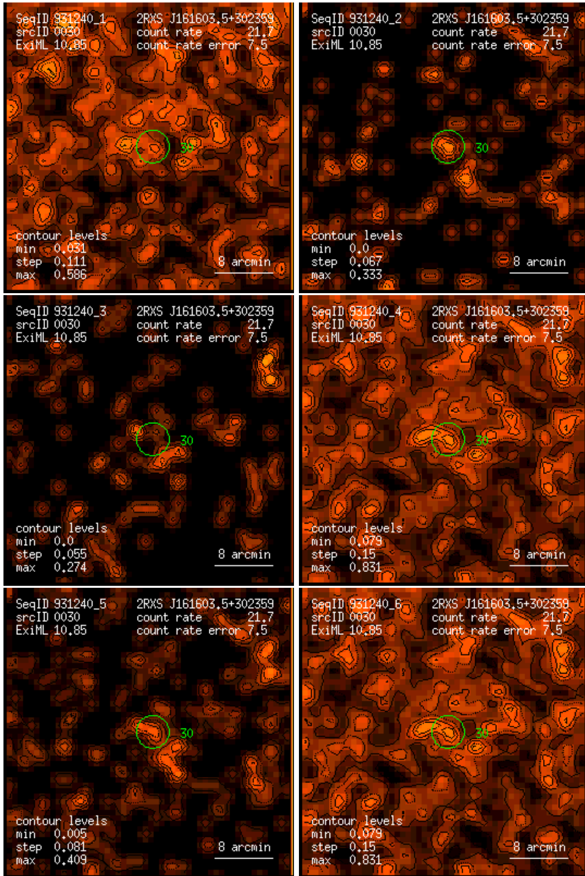
Figure 30: RASS 931240: detection 0030: band rate images, Gaussian filter: (1) PSPC channels 11 – 41, (2) 52 – 90, (3) 91 – 201, (4) 11 – 235, (5) 52 – 201, (6) 11 – 201. Broad band rates in counts/ks. Band rate contour levels in counts/ks/arcmin 2 .
