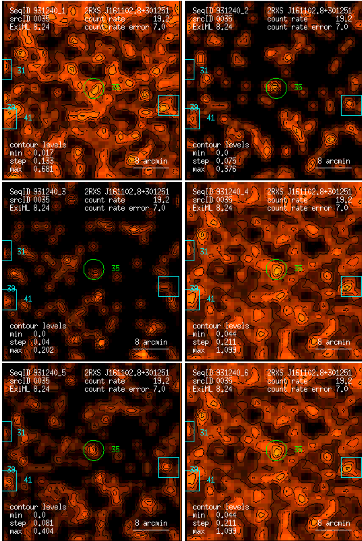
Figure 35: RASS 931240: detection 0035: band rate images, Gaussian filter: (1) PSPC channels 11 – 41, (2) 52 – 90, (3) 91 – 201, (4) 11 – 235, (5) 52 – 201, (6) 11 – 201. Broad band rates in counts/ks. Band rate contour levels in counts/ks/arcmin 2 .
