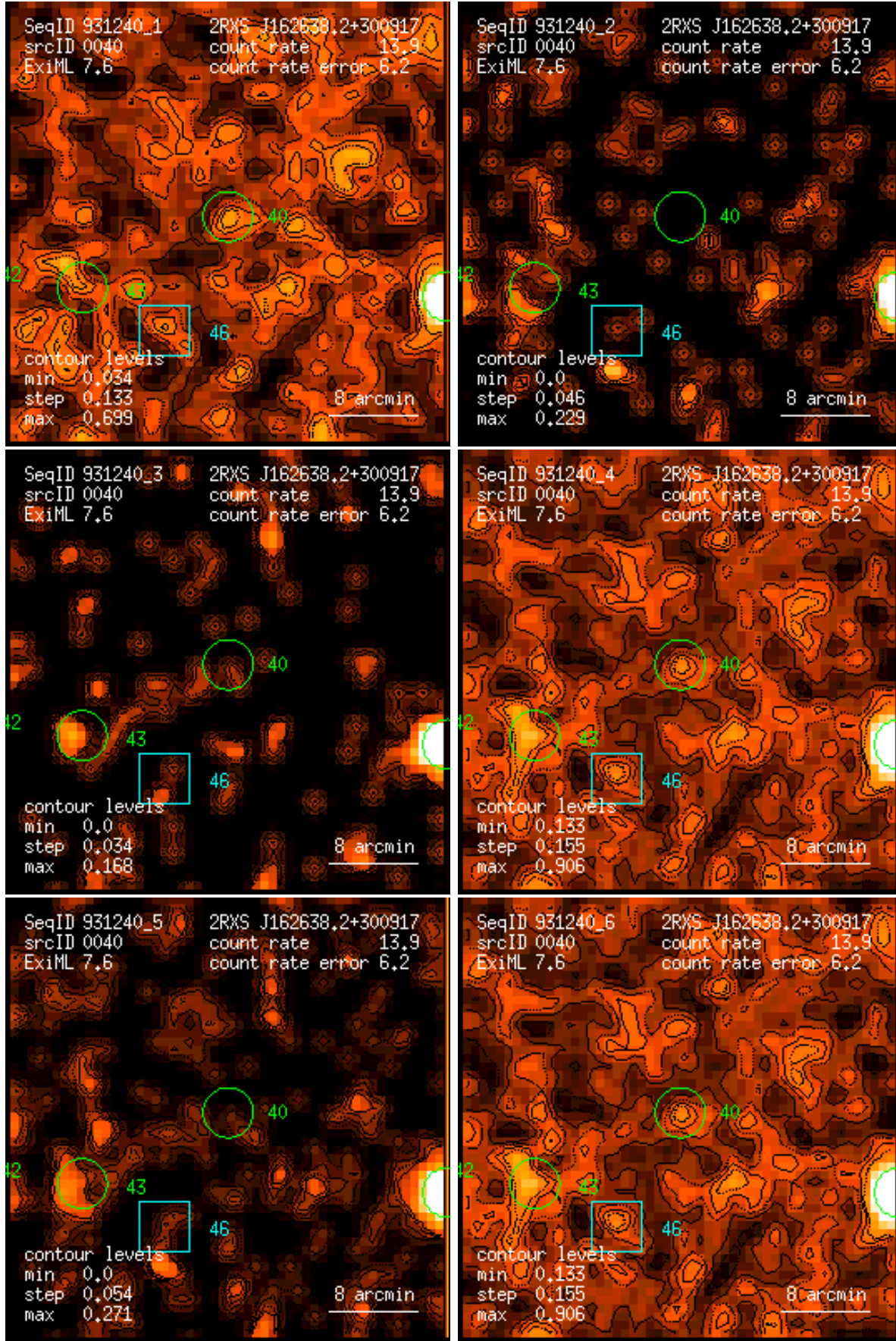
Figure 40: RASS 931240: detection 0040: band rate images, Gaussian filter: (1) PSPC channels 11 – 41, (2) 52 – 90, (3) 91 – 201, (4) 11 – 235, (5) 52 – 201, (6) 11 – 201. Broad band rates in counts/ks. Band rate contour levels in counts/ks/arcmin 2 .
