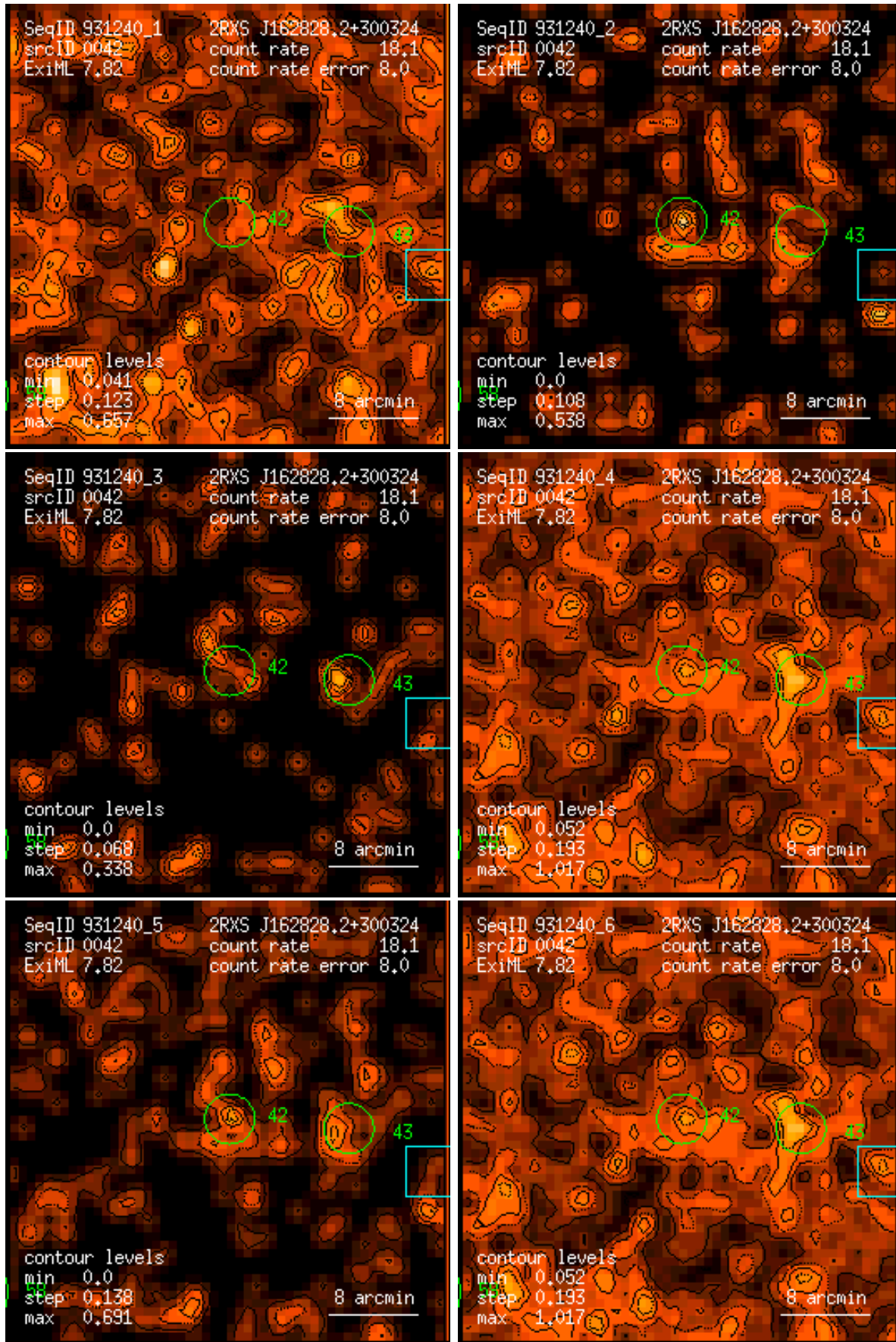
Figure 42: RASS 931240: detection 0042: band rate images, Gaussian filter: (1) PSPC channels 11 – 41, (2) 52 – 90, (3) 91 – 201, (4) 11 – 235, (5) 52 – 201, (6) 11 – 201. Broad band rates in counts/ks. Band rate contour levels in counts/ks/arcmin 2 .
