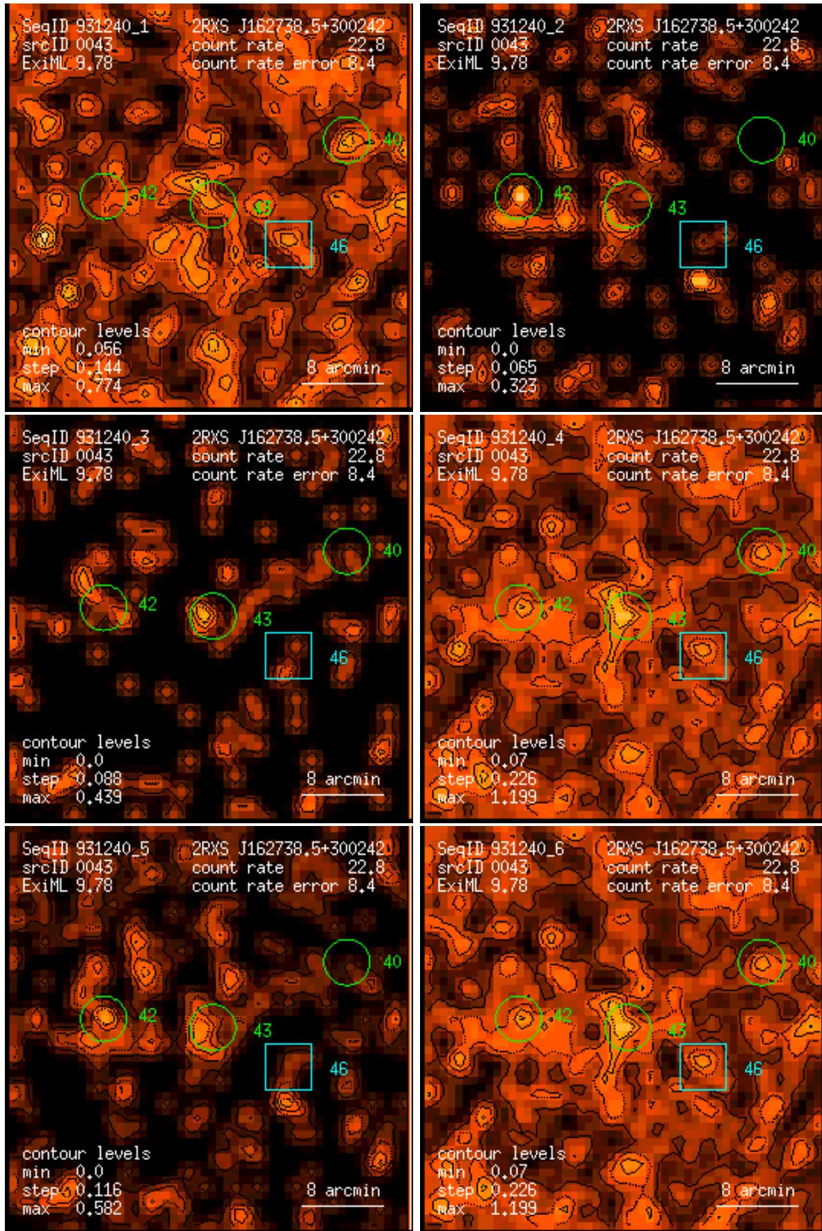
Figure 43: RASS 931240: detection 0043: band rate images, Gaussian filter: (1) PSPC channels 11 – 41, (2) 52 – 90, (3) 91 – 201, (4) 11 – 235, (5) 52 – 201, (6) 11 – 201. Broad band rates in counts/ks. Band rate contour levels in counts/ks/arcmin 2 .
