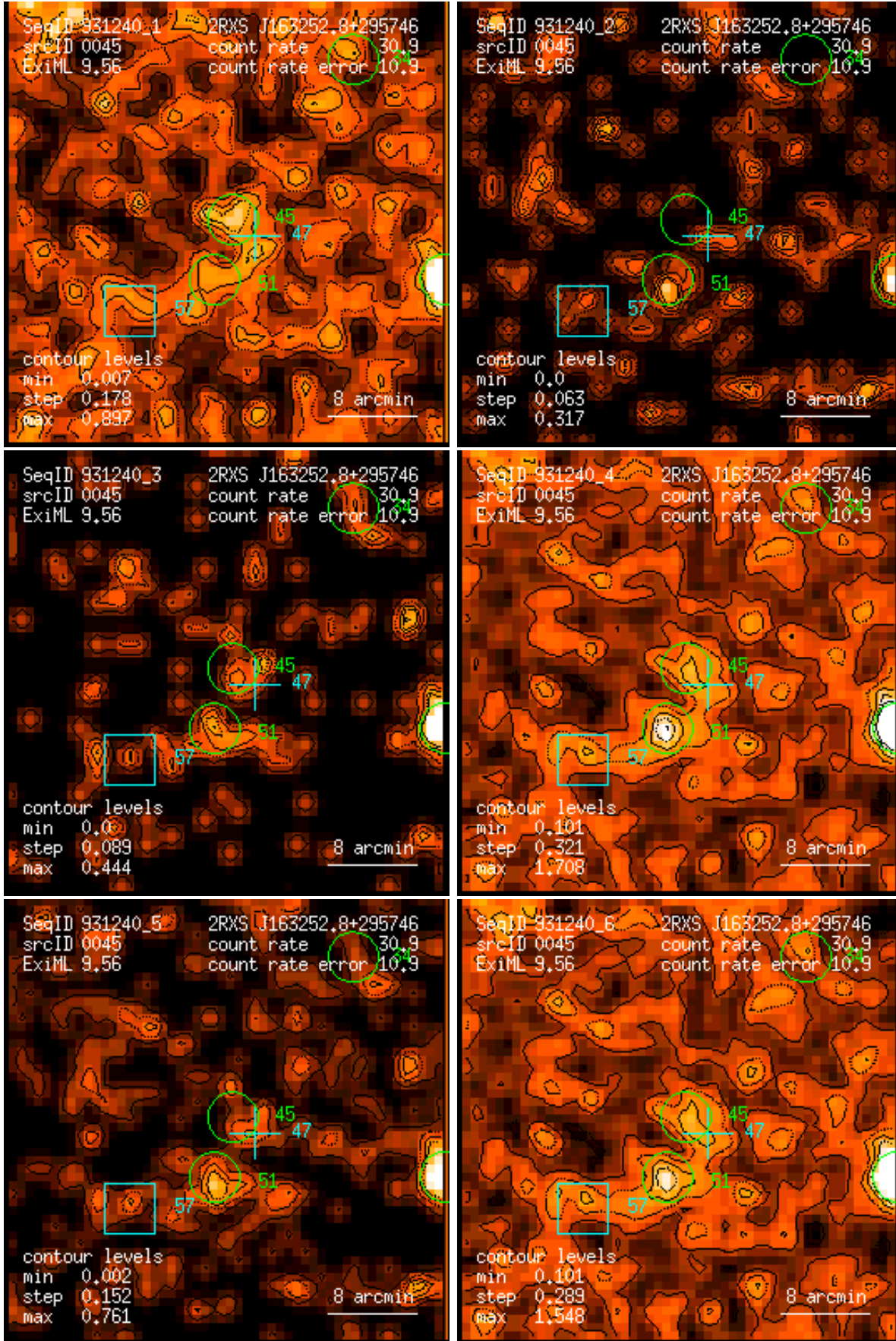
Figure 45: RASS 931240: detection 0045: band rate images, Gaussian filter: (1) PSPC channels 11 – 41, (2) 52 – 90, (3) 91 – 201, (4) 11 – 235, (5) 52 – 201, (6) 11 – 201. Broad band rates in counts/ks. Band rate contour levels in counts/ks/arcmin 2 .
