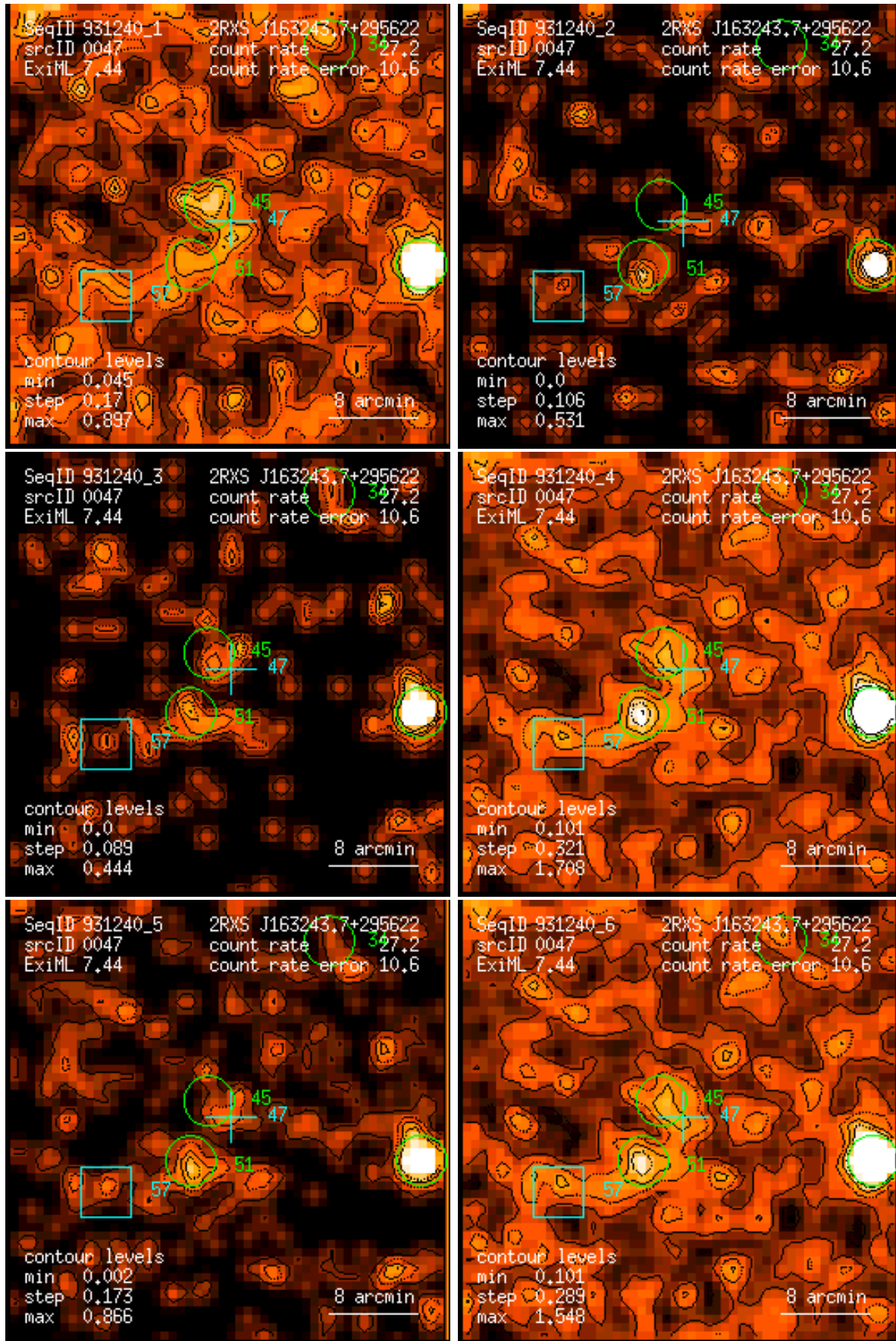
Figure 47: RASS 931240: detection 0047: band rate images, Gaussian filter: (1) PSPC channels 11 – 41, (2) 52 – 90, (3) 91 – 201, (4) 11 – 235, (5) 52 – 201, (6) 11 – 201. Broad band rates in counts/ks. Band rate contour levels in counts/ks/arcmin 2 .
