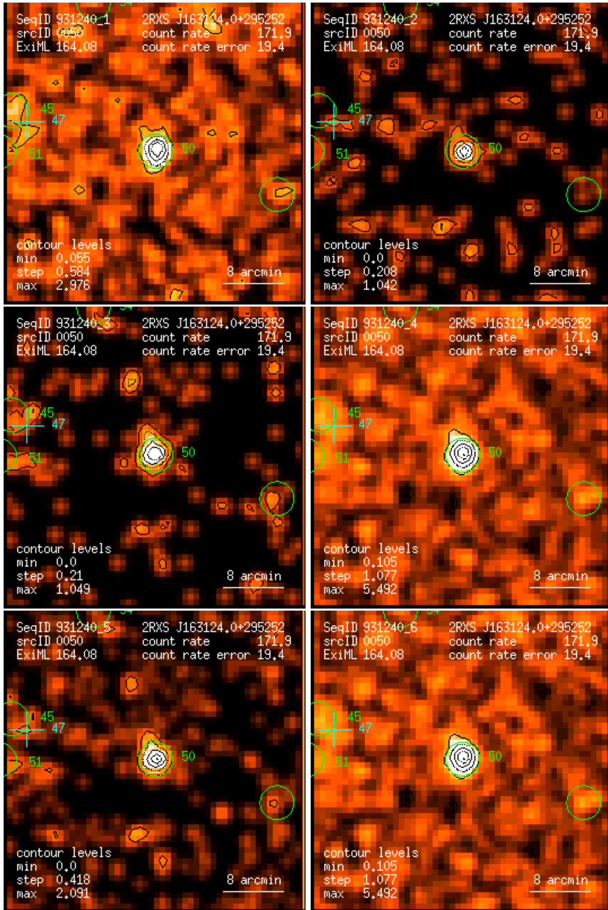
Figure 50: RASS 931240: detection 0050: band rate images, Gaussian filter: (1) PSPC channels 11 – 41, (2) 52 – 90, (3) 91 – 201, (4) 11 – 235, (5) 52 – 201, (6) 11 – 201. Broad band rates in counts/ks. Band rate contour levels in counts/ks/arcmin 2 .
