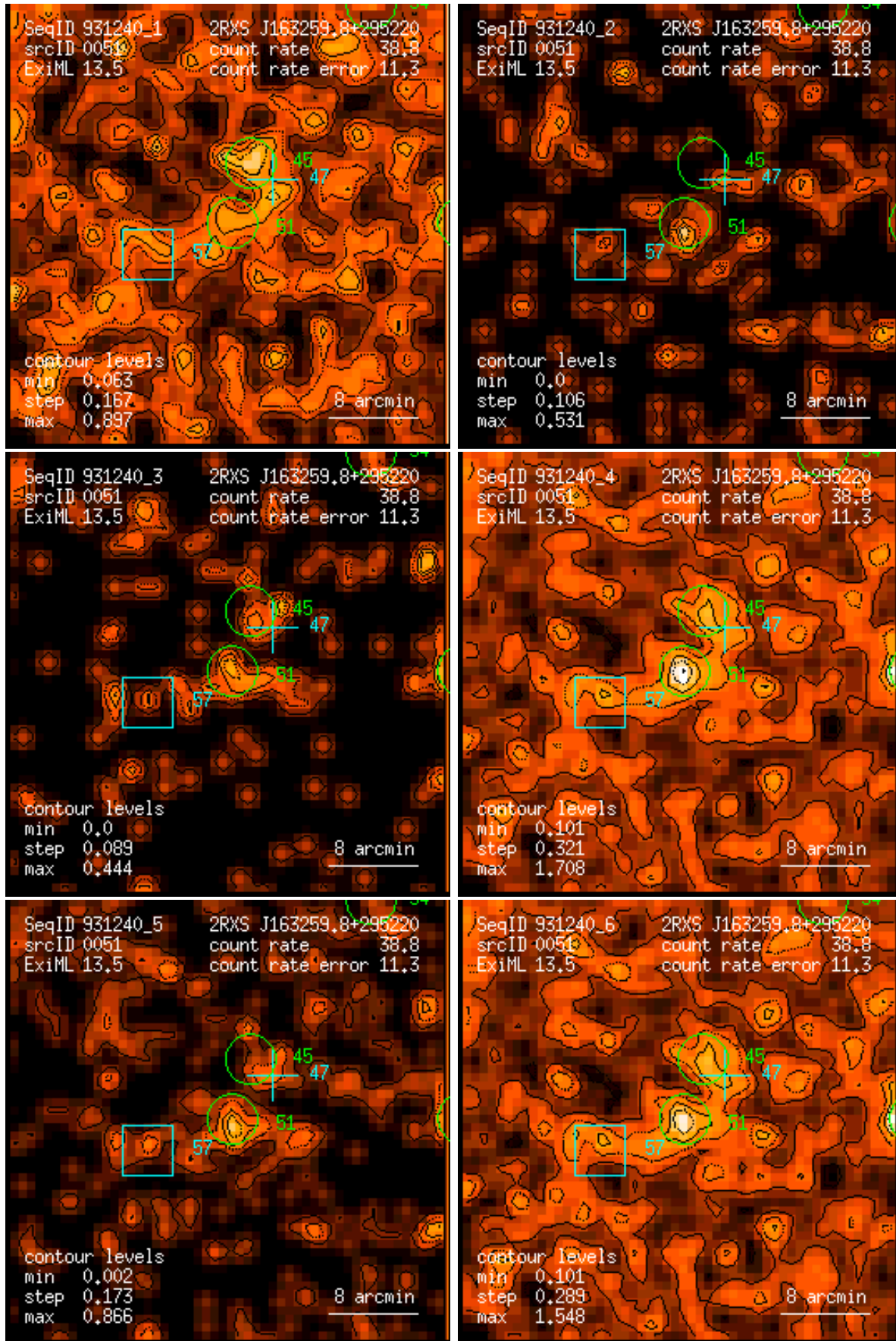
Figure 51: RASS 931240: detection 0051: band rate images, Gaussian filter: (1) PSPC channels 11 – 41, (2) 52 – 90, (3) 91 – 201, (4) 11 – 235, (5) 52 – 201, (6) 11 – 201. Broad band rates in counts/ks. Band rate contour levels in counts/ks/arcmin 2 .
