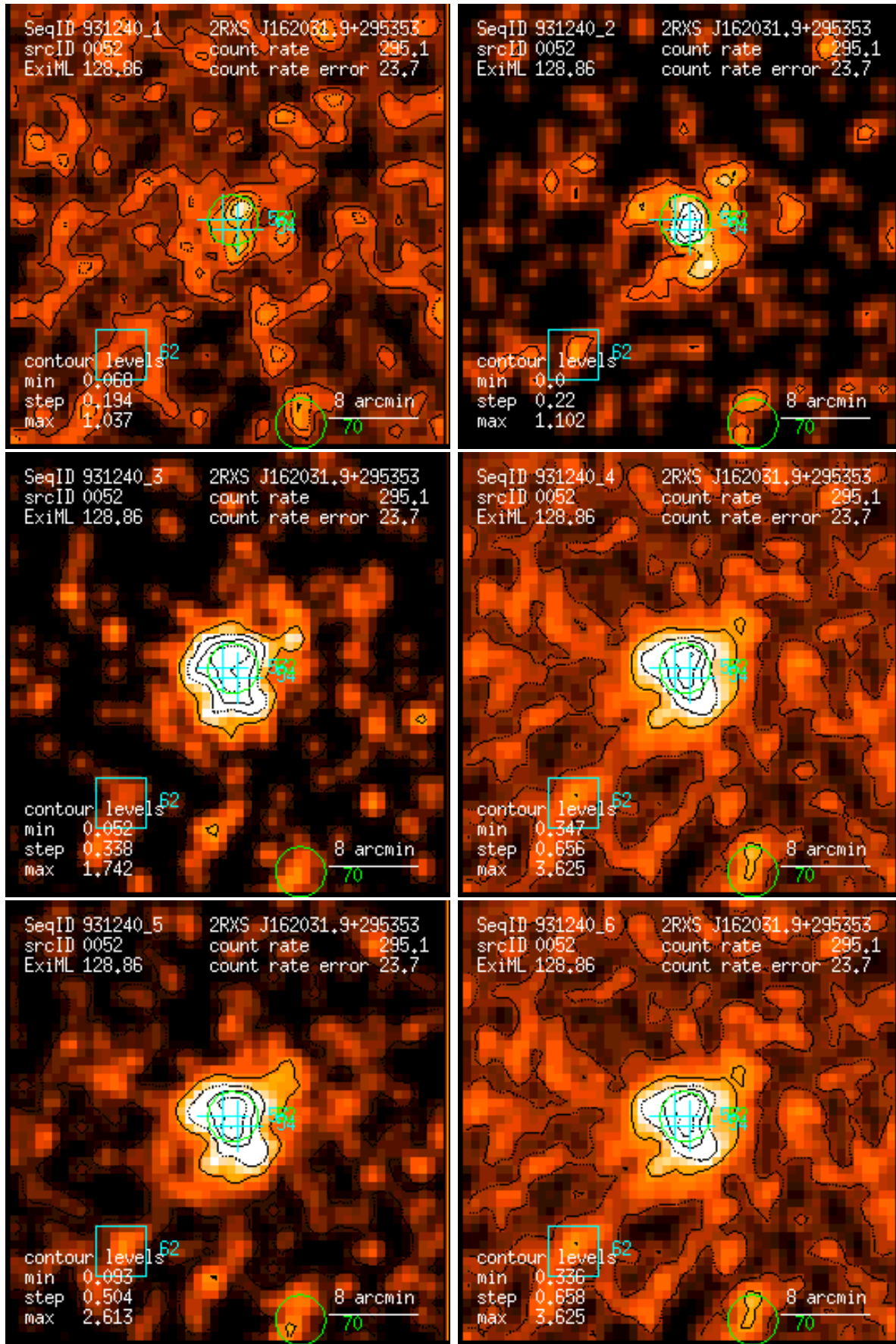
Figure 52: RASS 931240: detection 0052: band rate images, Gaussian filter: (1) PSPC channels 11 – 41, (2) 52 – 90, (3) 91 – 201, (4) 11 – 235, (5) 52 – 201, (6) 11 – 201. Broad band rates in counts/ks. Band rate contour levels in counts/ks/arcmin 2 .
