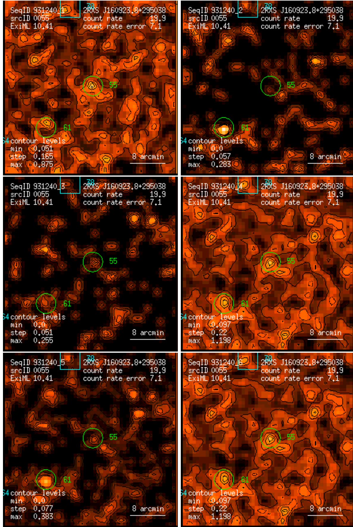
Figure 55: RASS 931240: detection 0055: band rate images, Gaussian filter: (1) PSPC channels 11 – 41, (2) 52 – 90, (3) 91 – 201, (4) 11 – 235, (5) 52 – 201, (6) 11 – 201. Broad band rates in counts/ks. Band rate contour levels in counts/ks/arcmin 2 .
