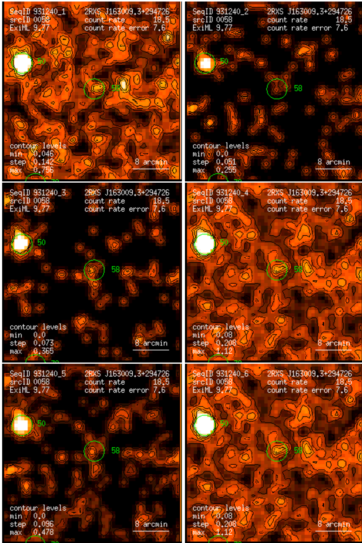
Figure 58: RASS 931240: detection 0058: band rate images, Gaussian filter: (1) PSPC channels 11 – 41, (2) 52 – 90, (3) 91 – 201, (4) 11 – 235, (5) 52 – 201, (6) 11 – 201. Broad band rates in counts/ks. Band rate contour levels in counts/ks/arcmin 2 .
