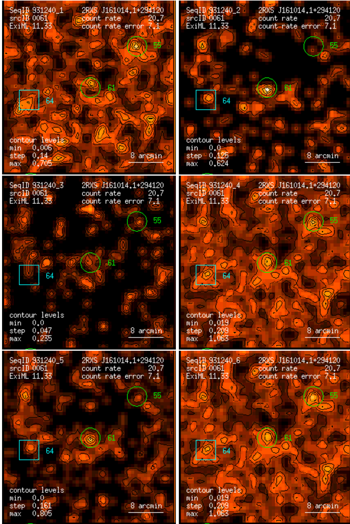
Figure 61: RASS 931240: detection 0061: band rate images, Gaussian filter: (1) PSPC channels 11 – 41, (2) 52 – 90, (3) 91 – 201, (4) 11 – 235, (5) 52 – 201, (6) 11 – 201. Broad band rates in counts/ks. Band rate contour levels in counts/ks/arcmin 2 .
